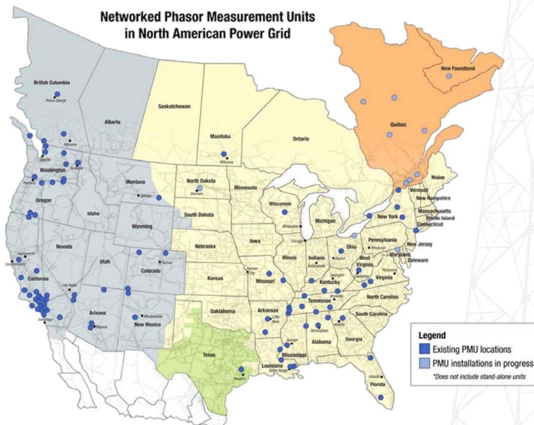
Figure 3.16. Networked Phasor Measurement Units in the North American Power Grid (PNNL/EIOC 2008)
