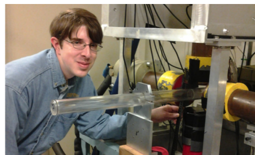
Figure 1. A 3D rendering (left) of the experimental setup used for the NRF measurements and a photograph (right) of the setup with Brent Fallin, one of the graduate students in the collaboration. High-purity Germanium detectors are placed around the target to determine the \gamma -ray emission pattern.
