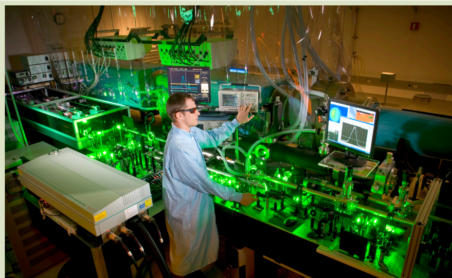
Figure 1. The Texas Petawatt Laser amplifier bay during Petawatt operations.
