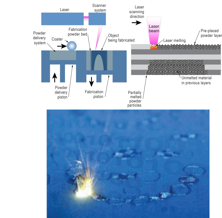
Figure 1. Laser powder bed fusion metal additive manufacturing. In metal powder bed fusion, a layer of metal powder is spread on a powder bed and melted using a laser. When the layer is complete, the fabrication piston moves downward by the thickness of one layer, the delivery piston moves up, and the coater is used to spread the next layer. This process is repeated hundreds to thousands of times until a complete part is fabricated.
