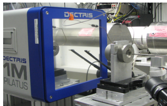
Figure 2. Fast compression/decompression experiments at HPCAT (currently to ~17 TPa per second) bridge the gap between conventional static and dynamic compression.
