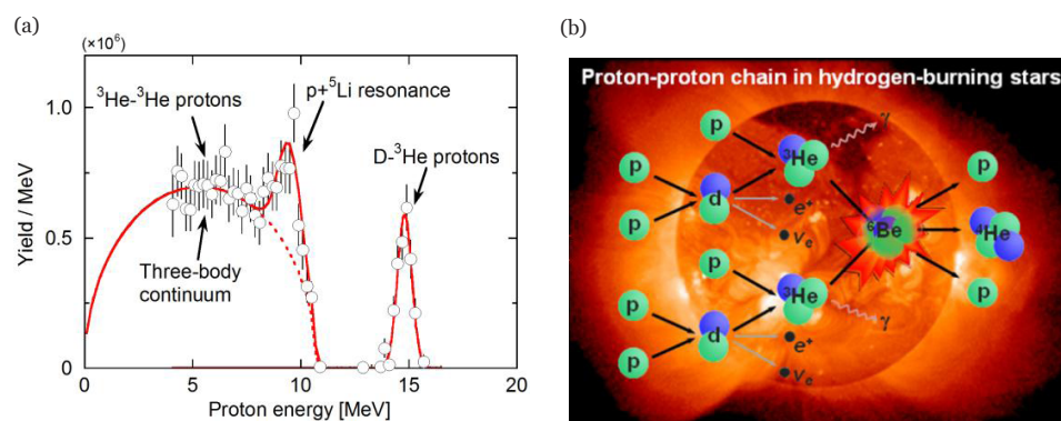
Figure 2. (a) The first preliminary {}^3\text{He} - {}^3\text{He} proton spectrum ever obtained using a plasma (OMEGA shot 61252, with a {}^3\text{He} -gas-filled exploding pusher), measured with MIT-developed compact proton spectrometers. Both the three-body continuum and the p+{}^5\text{Li} resonance at 9.3 MeV are observed at an average Gamow energy of \sim 95 keV. This measurement is directly relevant to first-generation, hydrogen-burning Population III stars, which were responsible for the first synthesis of heavy nuclei in the universe. Understanding the evolution of these stars will be critical for calculations of later stellar and galactic dynamics. (b) The proton-proton (pp) chain that took place in Population III stars, at conditions very similar to those in our {}^3\text{He} - {}^3\text{He} experiments, also takes place in hydrogen-burning stars like our Sun. These stars were responsible for the first synthesis of heavy nuclei in the universe. Understanding their evolution will be critical for calculations of later stellar and galactic dynamics. These stars will be studied by other groups using the James Webb Space Telescope.
