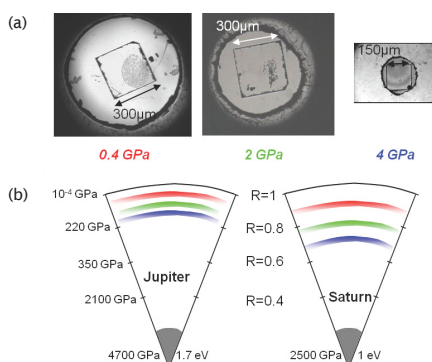
Figure 1. (a) Change in pressure-chamber dimensions within the diamond anvil cell targets, documenting how design improvements over the past years allow higher precompressions than ever. (b) Achieving higher precompression allows studying fluids at pressure-density-temperature conditions relevant for deep regions inside Jupiter and Saturn: the color scale relates the initial pressure to the depth within the planets that can now be recreated using OMEGA.
