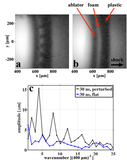
Figure 2. Data and analysis from the RM experiment. Parts (a) and (b) show data from shots with and without the machined seed perturbation, respectively. Both images were taken roughly 13 ns after the shock crosses the foam/plastic interface. Part (c) shows the Fourier transform of the foam/plastic interface contour, demonstrating the growth of the initial modes of wavenumber k=4 and k=8 , corresponding to 100 \mu\text{m} and 50 \mu\text{m} wavelengths, respectively, as well as the appearance of harmonic modes k=4+8=12 and k=12+4=16 , corresponding to wavelengths of 33 \mu\text{m} and 25 \mu\text{m} , respectively.
