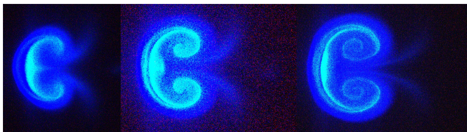
Figure 1. Mosaic of experimental images showing laser-induced fluorescence in planar cross-sections of a Mach 1.7 shock-accelerated \text{SF}_6 column. Flow direction is from left to right, vertical image extent is 16 mm, timings after shock arrival are 50, 100, and 150 \mu\text{s} .
