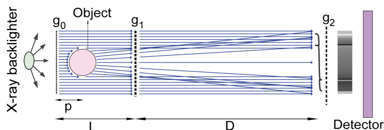
Figure 1. The essential elements of a high magnification Talbot-Lau interferometer; typical L \sim 25 cm and D \sim 100 cm.
