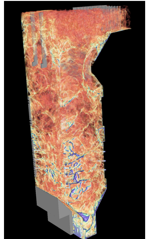
A volume rendered image of a CCMSC prediction of an Alstom oxycoal boiler. The image shows local concentrations of the 90 micron coal particles in the boiler. The particles concentrate in local regions due to variation in local Stokes number. The simulation was performed on Titan using 1 million core hours.
