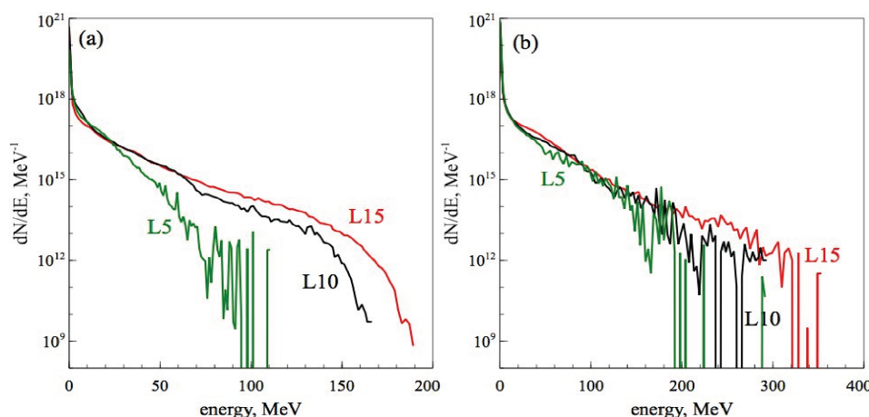
Figure 1. Numerically-simulated time integrated energy spectra of fast electrons passing through the extraction plane and entering the solid target with three different pre-plasma scale lengths (green: L = 5 , black: L = 10 , and red: L = 15 \mu\text{m} ), for laser pulse duration of 1 ps (Figure 1a) and 3 ps (Figure 1b).
