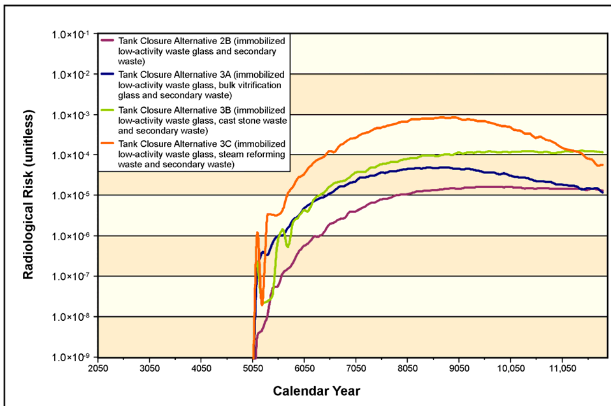
Figure S-15. Lifetime Radiological Risk for the Drinking-Water Well User at the 200-East Area Integrated Disposal Facility Barrier from Tank Closure Treatment Process-Generated Waste Forms
