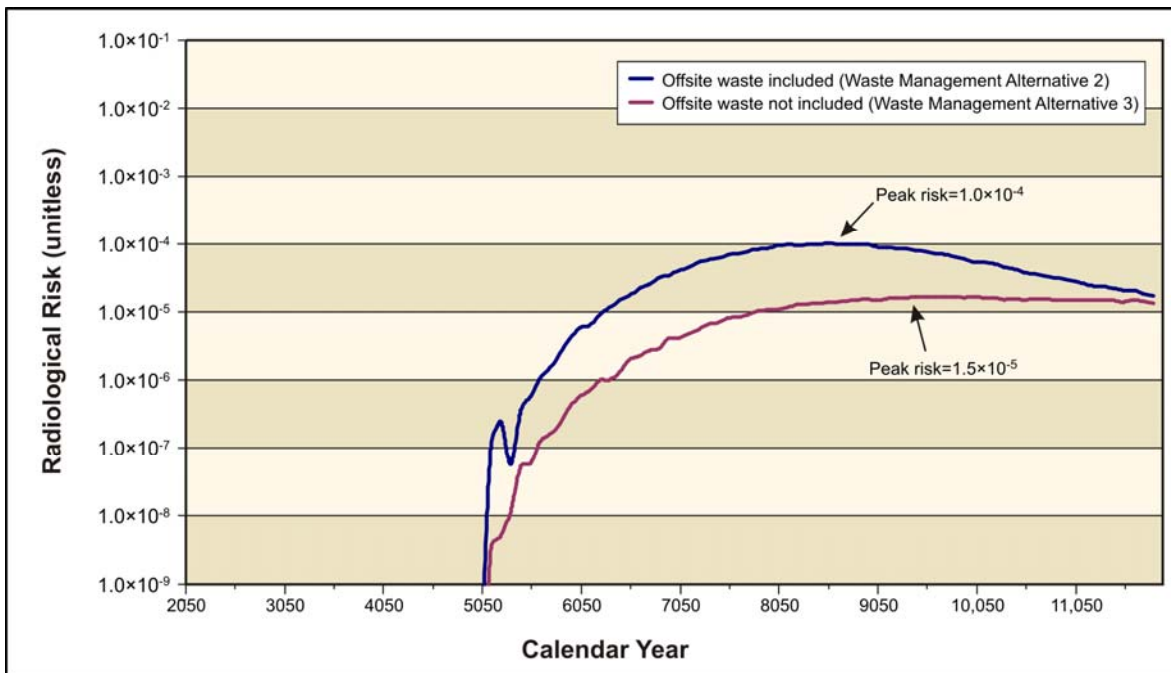
Figure S–21. Tank Closure Alternative 2B Lifetime Radiological Risk for the Drinking-Water Well User at the 200-East Area Integrated Disposal Facility Barrier
