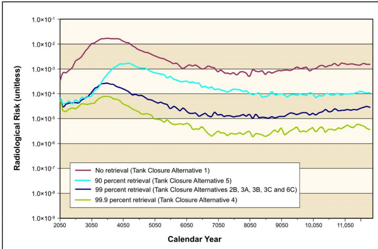
Figure S-14. Lifetime Radiological Risk for the Drinking-Water Well User at the Core Zone Boundary due to Releases from Tank Farm Residuals and Ancillary Equipment and to Retrieval Leaks
