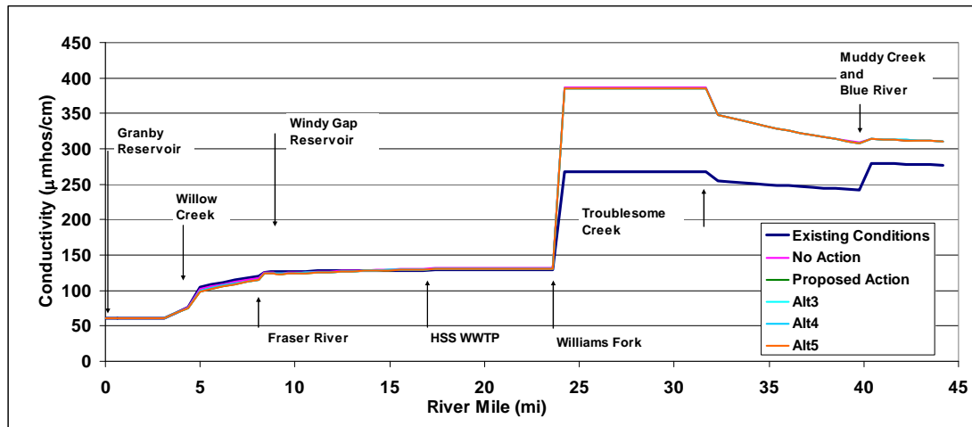
Figure 3-57. Colorado River specific conductivity for July 25 assuming diversion to the minimum streamflow below Windy Gap Reservoir.
