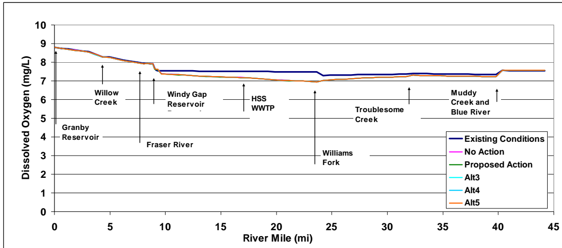
Figure 3-59. Colorado River dissolved oxygen concentrations for July 25 assuming diversion to the minimum streamflow below Windy Gap Reservoir.
