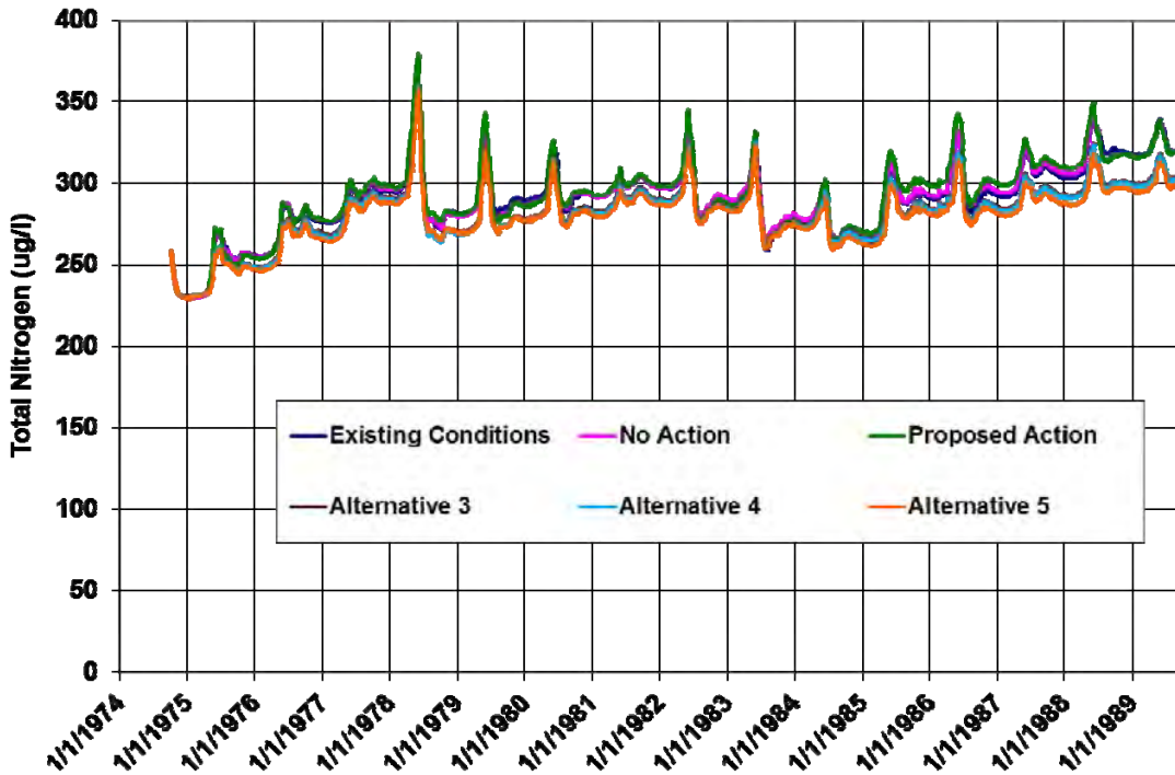
Figure 3-69. Simulated daily total nitrogen concentrations in Granby Reservoir (existing conditions and all alternatives).
