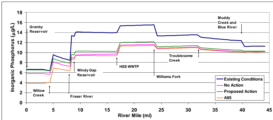
Figure 3-87. Colorado River inorganic phosphorus concentrations for July 25—cumulative effects.
