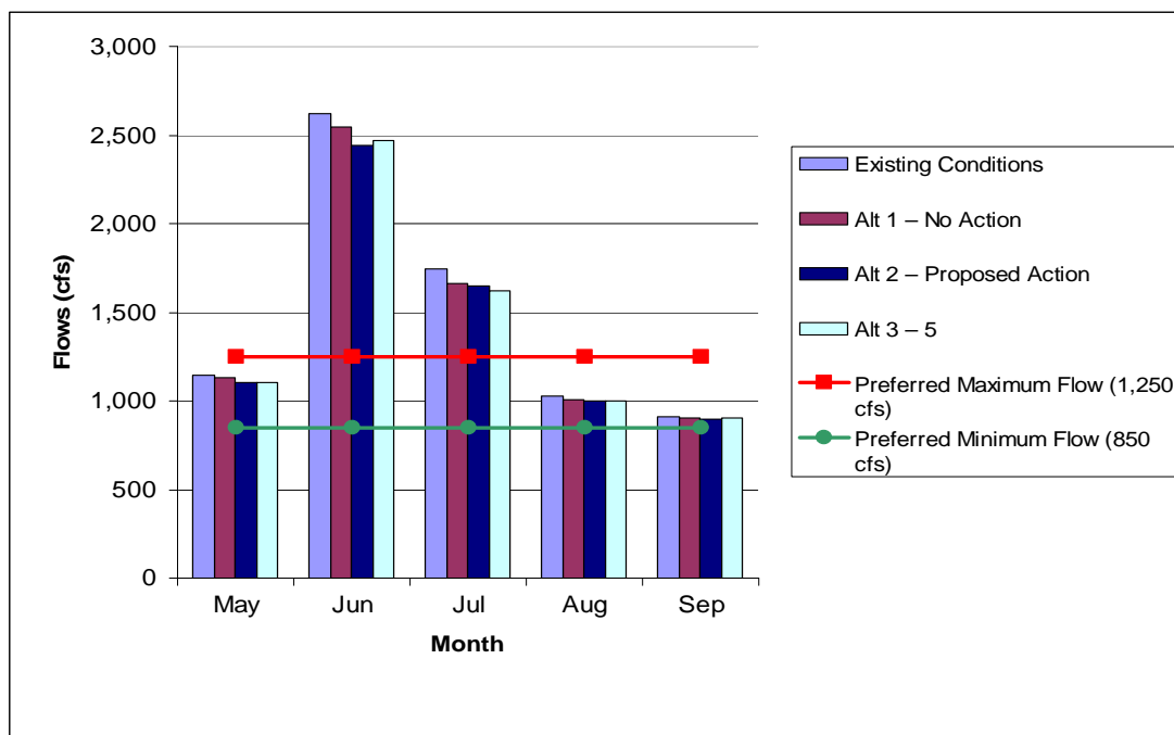
Figure 3-118. Average monthly streamflow on the Colorado River through Big Gore Canyon for rafting and kayaking.
