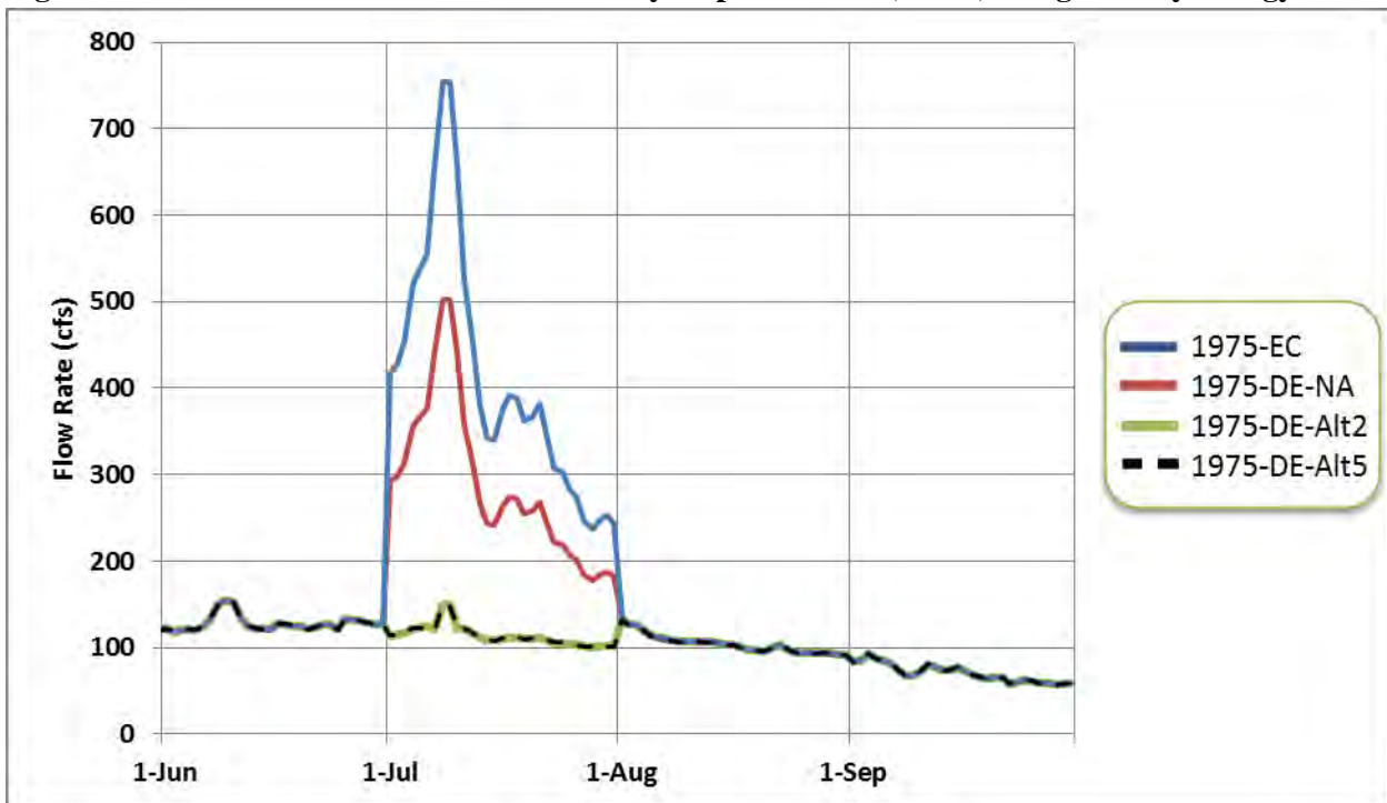
Figure 3-46. Colorado River flow below Windy Gap Reservoir (WGD) using 1975 hydrology.
