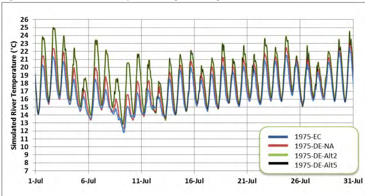
Figure 3-47. Colorado River hourly stream temperatures upstream of the Williams Fork (WFU).
