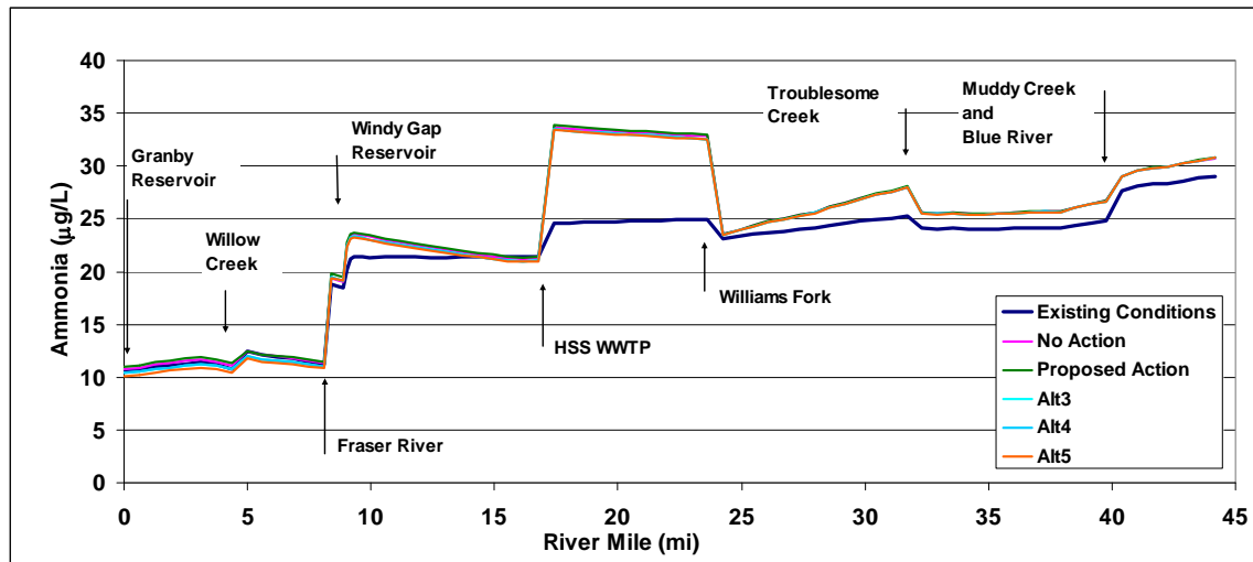
Figure 3-61. Colorado River ammonia concentrations for July 25 assuming diversion to the minimum streamflow below Windy Gap Reservoir.
