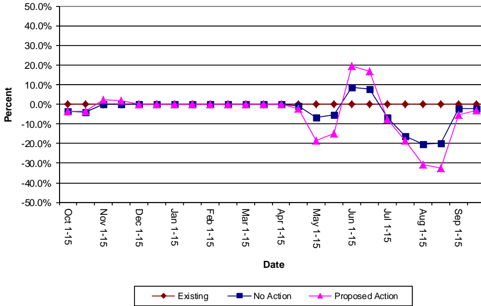
Figure 3-101. Percent change in adult brown trout habitat from existing conditions on the Colorado River below Windy Gap for an average water year.
