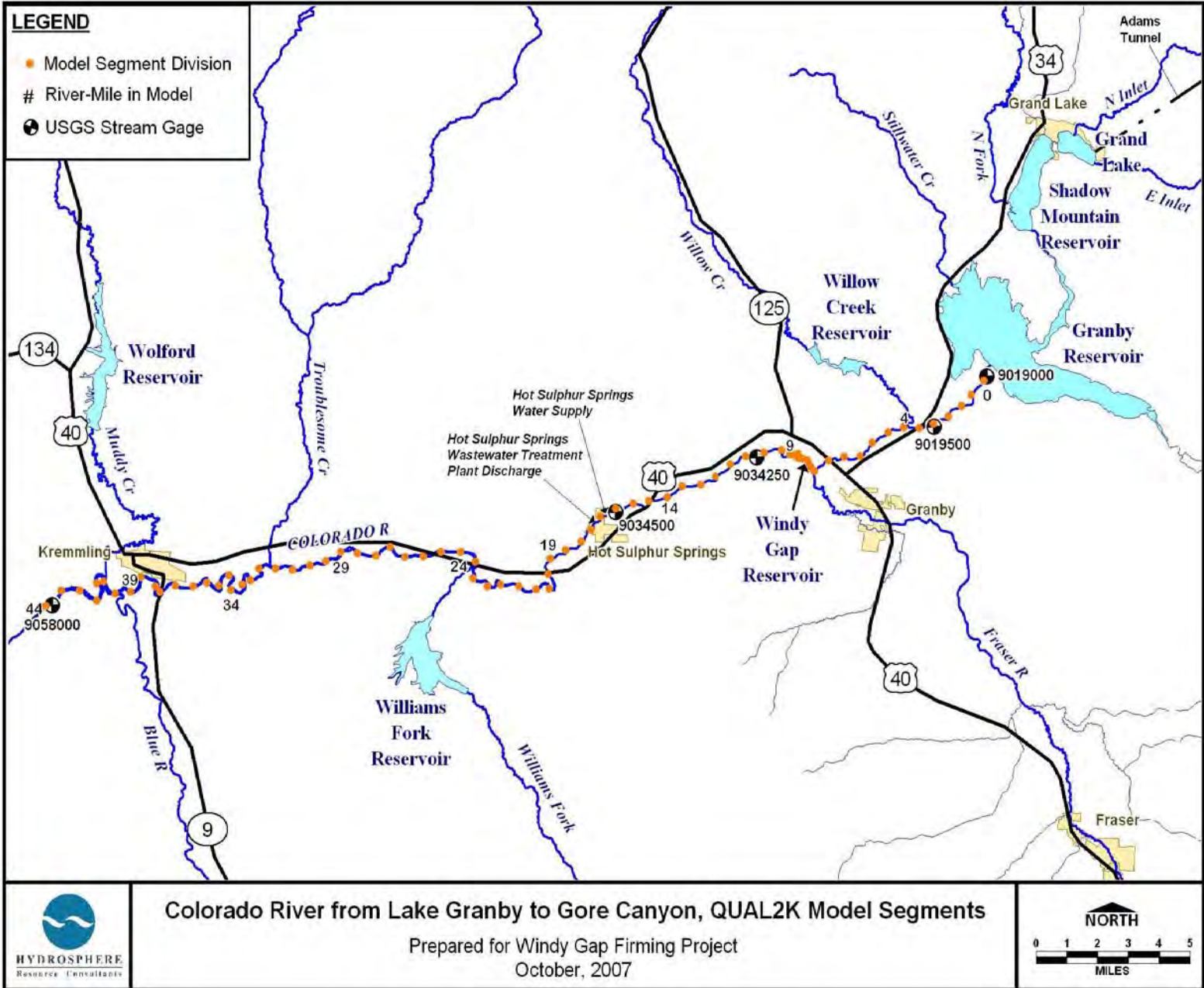
Figure 3-44. QUAL2K model segments, Colorado River from Granby Reservoir to Gore Canyon.
