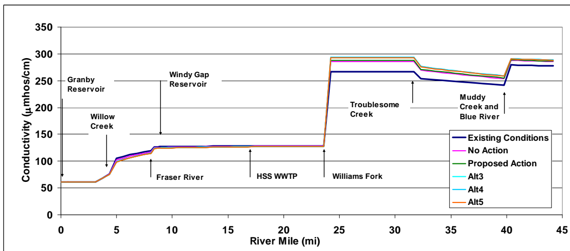
Figure 3-56. Colorado River specific conductivity for July 25.
