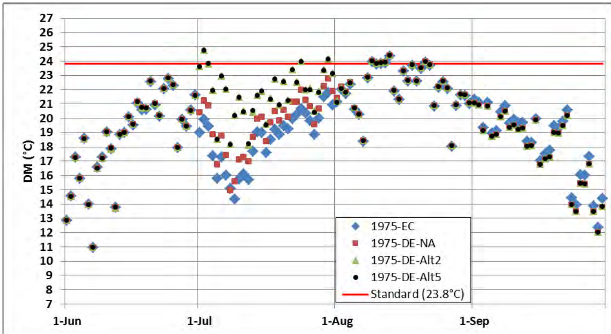
Figure 3-52. Daily Maximum Temperature at Colorado River at Hot Sulphur Springs (HSU), June to September 1975.
