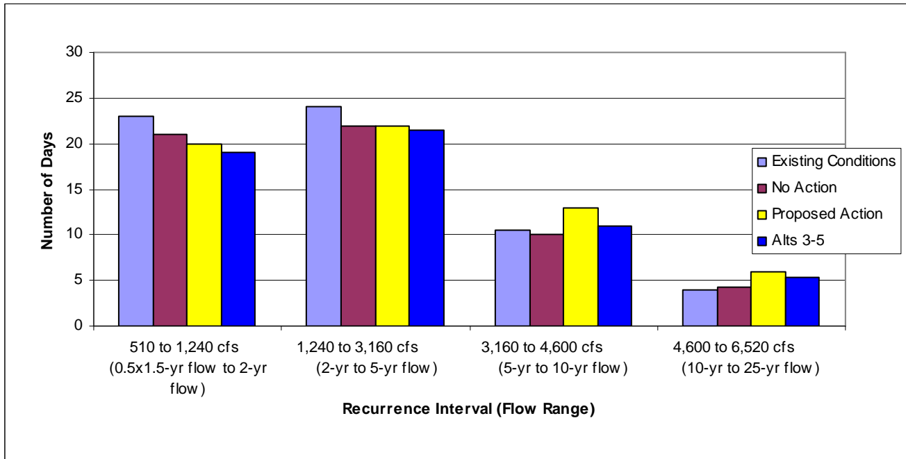
Figure 3-34. Duration of channel maintenance flows in years when such flows occur at Hot Sulphur Springs.
