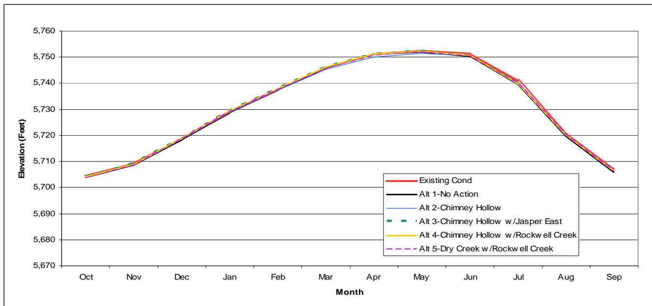
Figure 3-18. Carter Lake estimated average monthly surface elevation for all alternatives.
