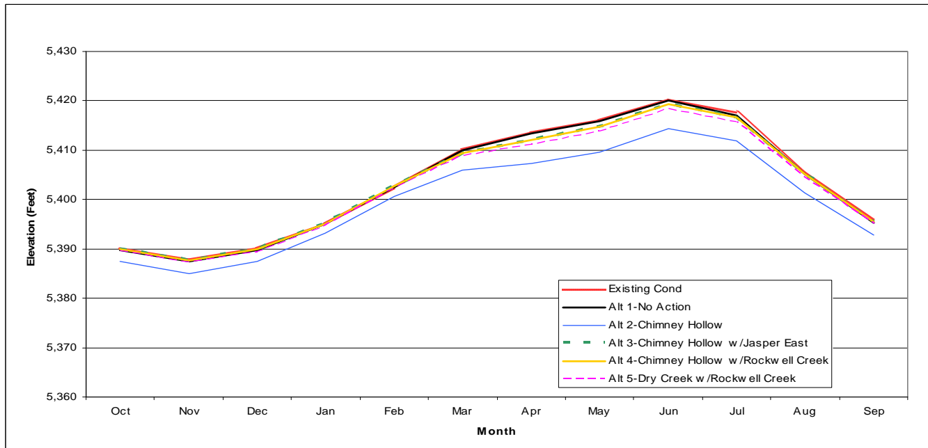
Figure 3-19. Horsetooth Reservoir estimated average monthly surface elevation for all alternatives.
