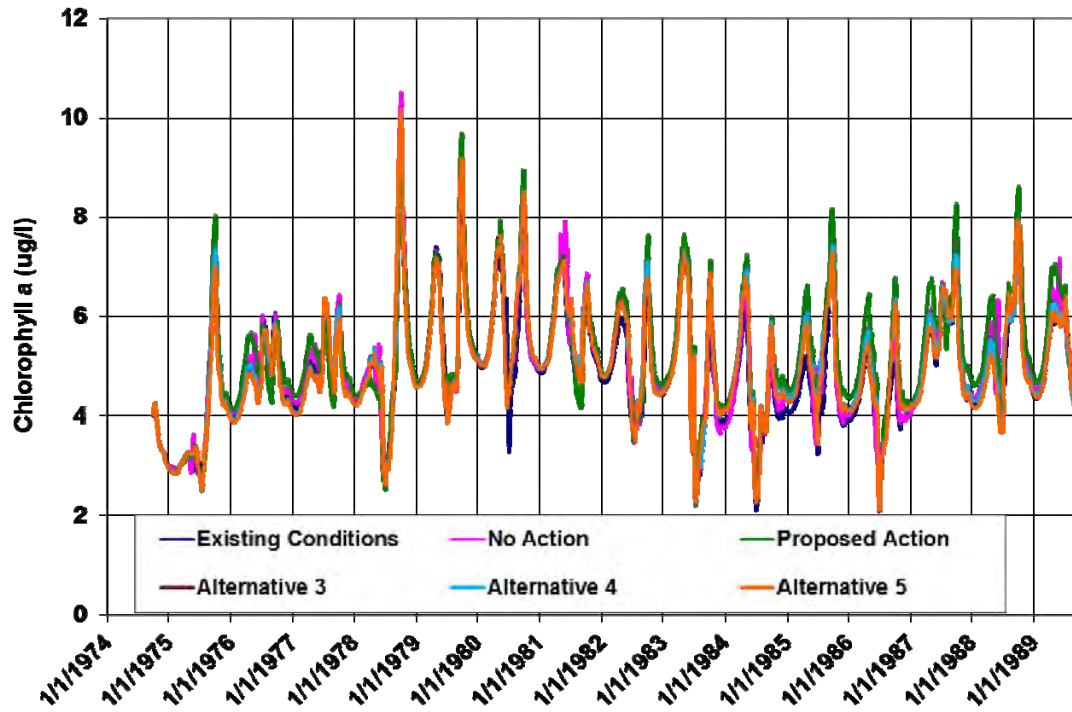
Figure 3-80. Simulated daily chlorophyll a concentrations in Grand Lake (existing conditions and all alternatives).
