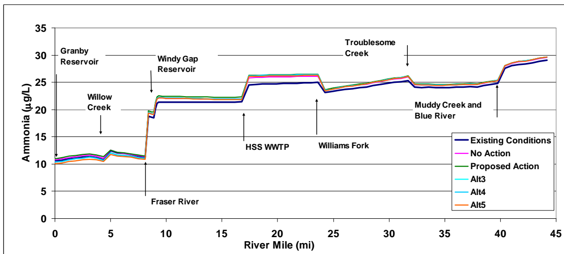
Figure 3-60. Colorado River ammonia concentrations for July 25.
