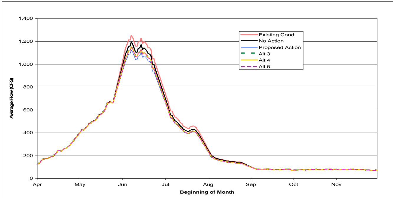
Figure 3-13. Colorado River above Windy Gap – average daily flows by alternative.
