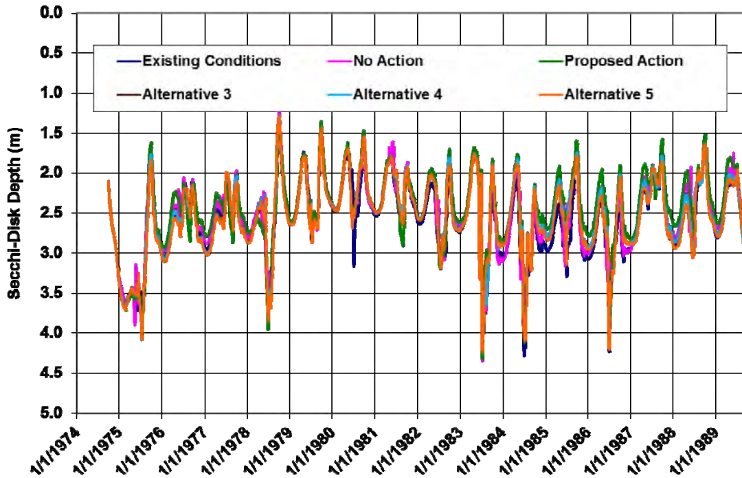
Figure 3-81. Simulated daily Secchi depth in Grand Lake (existing conditions and all alternatives).
