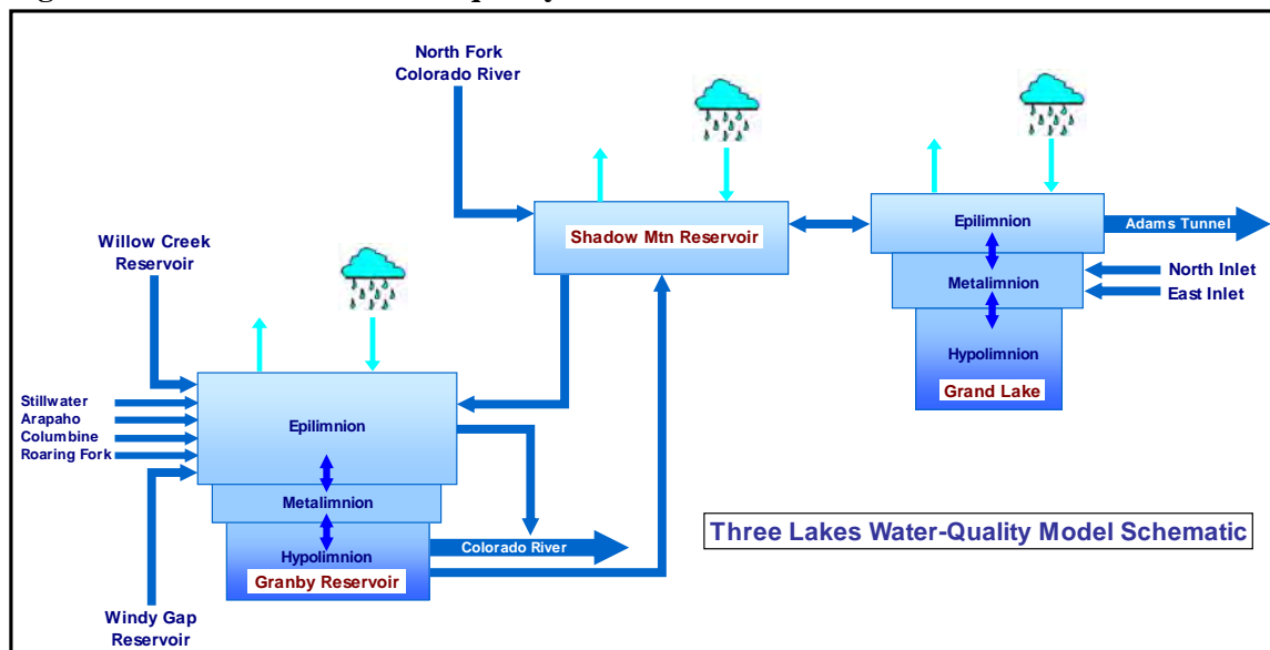
Figure 3-45. Three Lakes water quality model schematic.
