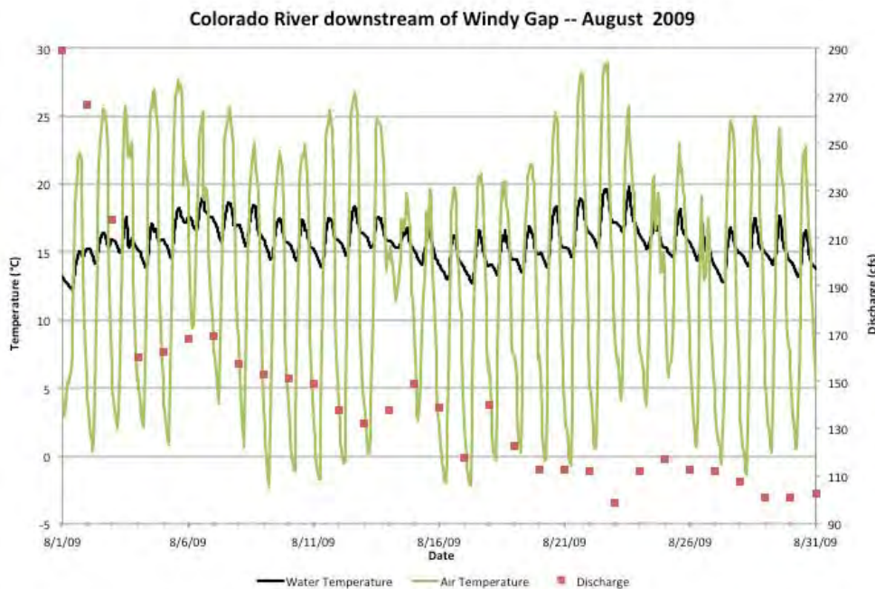
Figure 3-91. Hourly water temperatures, air temperature (at Granby), and mean daily discharge for the Colorado River downstream of Windy Gap Reservoir – August 2009.
