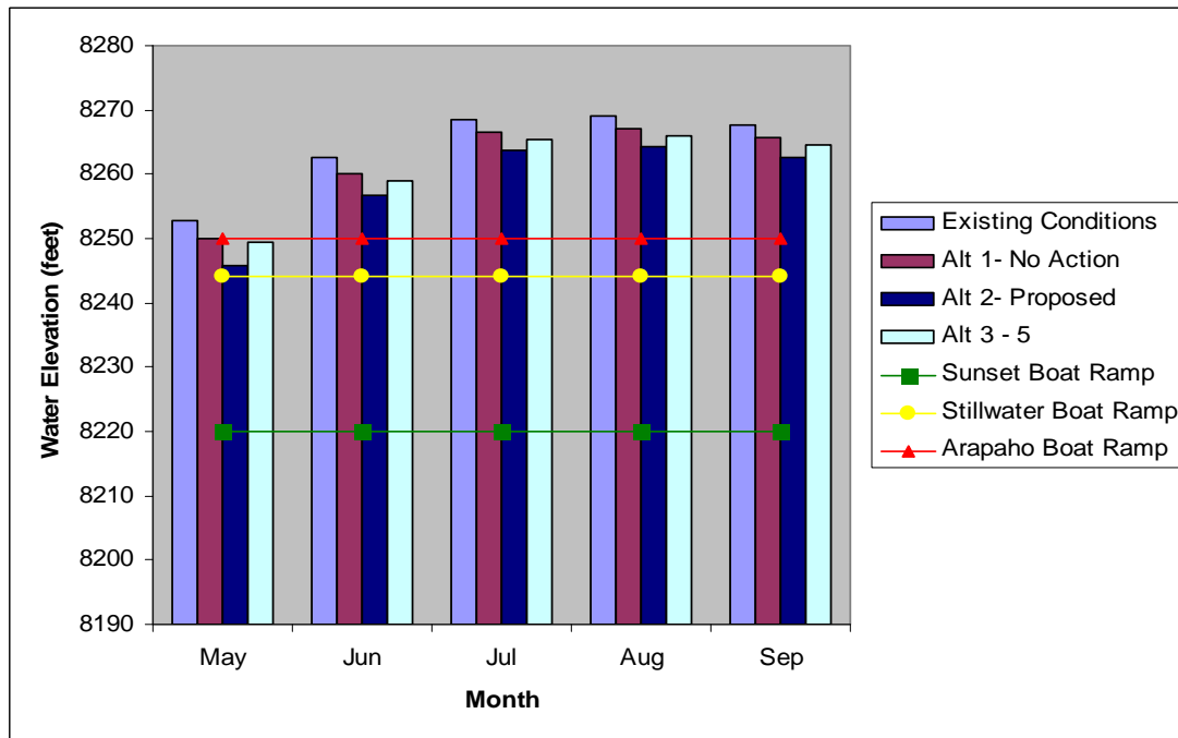
Figure 3-116. Average monthly water levels at Granby Reservoir boat ramps.
