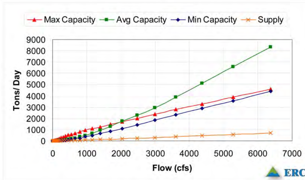
Figure 3-31. Comparison of sediment supply vs. transport capacity at CR-1, Colorado River above Parshall.
