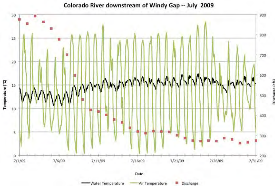
Figure 3-90. Hourly water temperatures, air temperature (at Granby), and mean daily discharge for the Colorado River downstream of Windy Gap Reservoir – July 2009.
