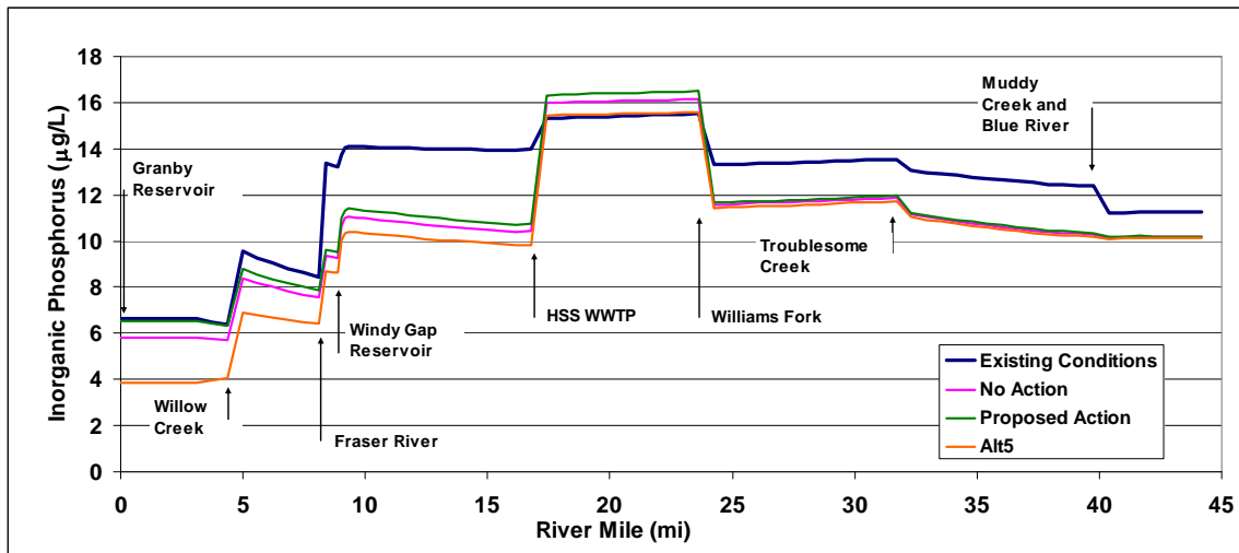
Figure 3-88. Colorado River inorganic phosphorus concentrations for July 25 assuming diversion to the minimum streamflow below Windy Gap Reservoir—cumulative effects.
