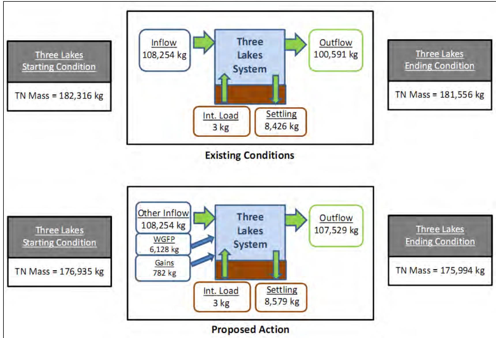
Figure 3-67. Fate of total nitrogen (TN) for the Three Lakes system (average annual kg/yr, WY75–WY89).
