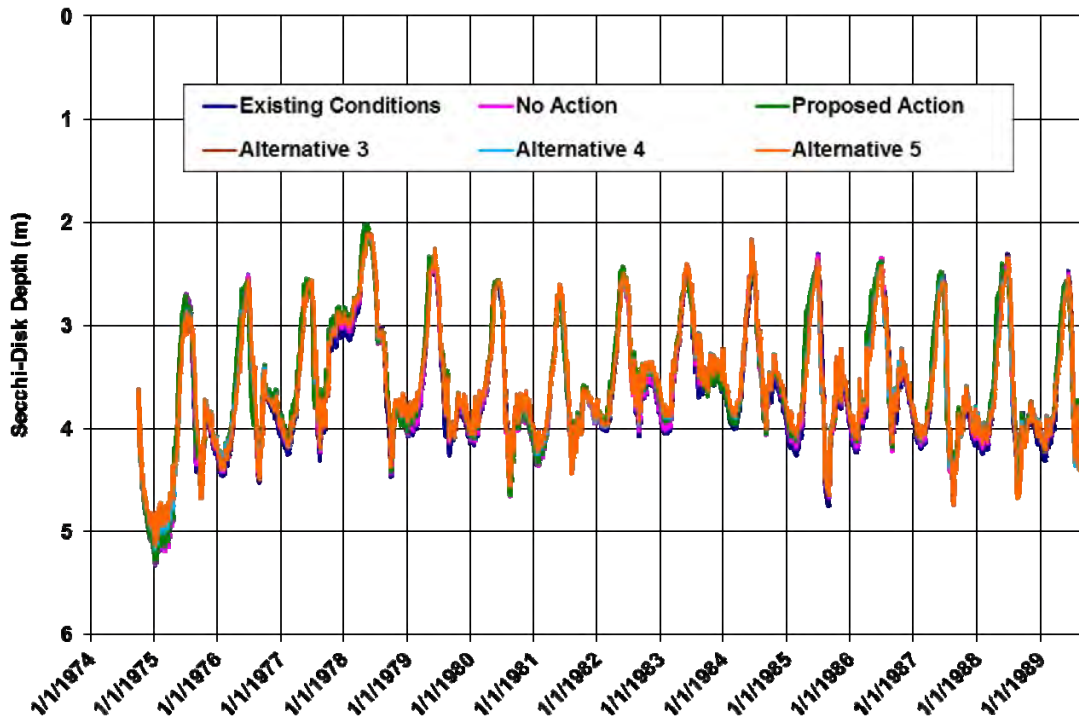
Figure 3-71. Simulated daily Secchi depth in Granby Reservoir (existing conditions and all alternatives).
