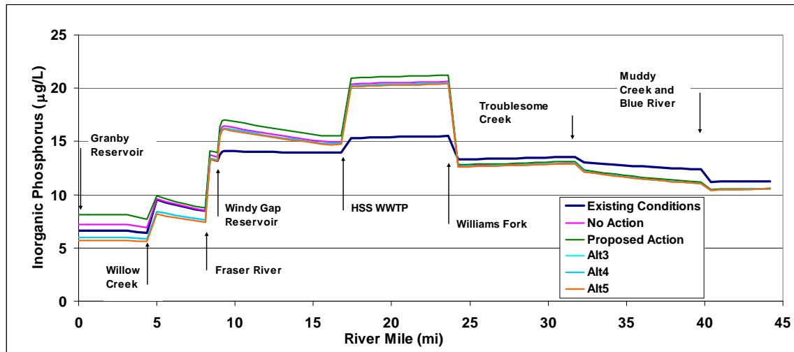
Figure 3-63. Colorado River inorganic phosphorus concentrations for July 25 assuming diversion to the minimum streamflow below Windy Gap Reservoir.
