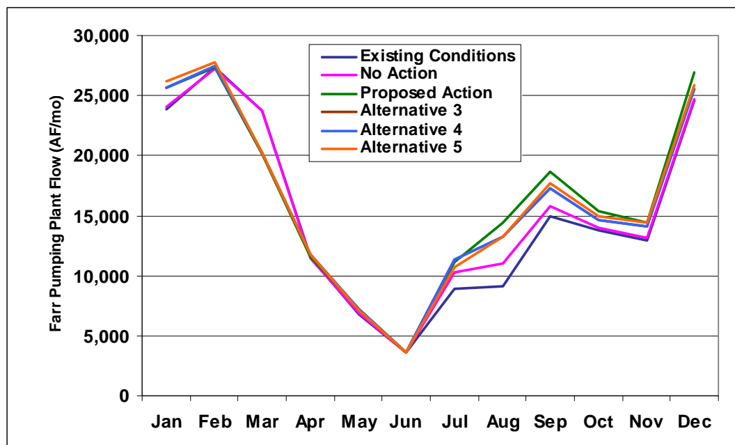
Figure 3-65. Estimated pumping from Granby Reservoir to Shadow Mountain Reservoir via the Farr Pumping Plant.
