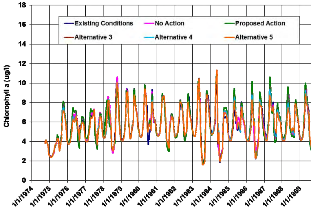
Figure 3-75. Simulated daily chlorophyll a concentrations in Shadow Mountain Reservoir (existing conditions and all alternatives).
