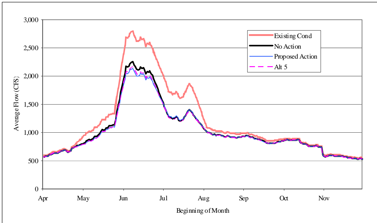
Figure 3-28. Colorado River near Kremmling – average daily flows with reasonably foreseeable actions.
