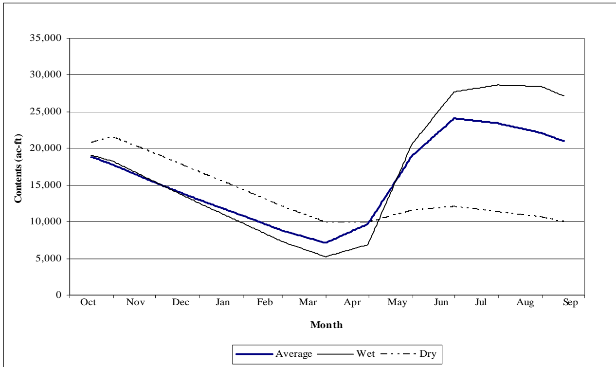
Figure 3-25. Rockwell Reservoir (30,000 AF) daily content under Alternative 5.
