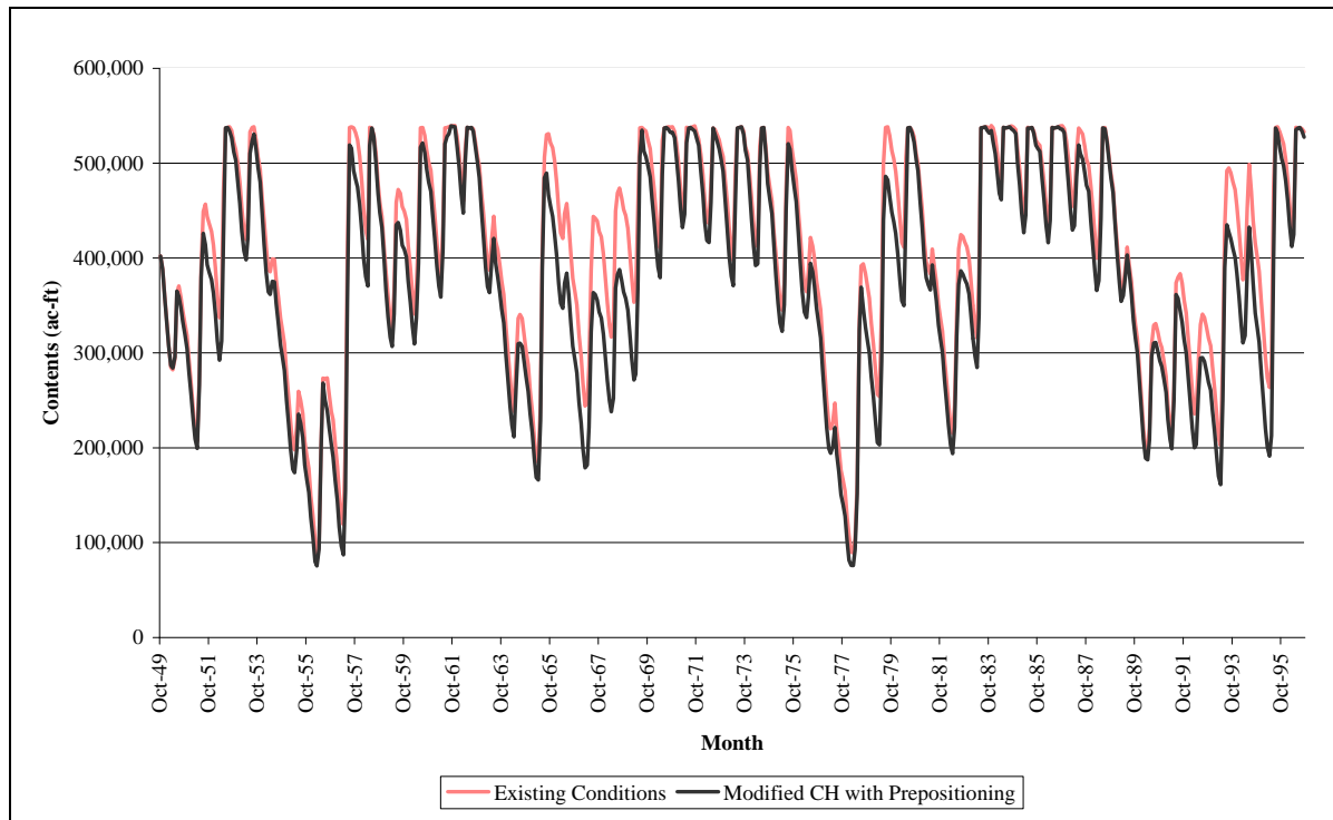
Figure 3-29. Comparison of monthly Granby Reservoir elevation for existing conditions and modified prepositioning under the Preferred Alternative.
