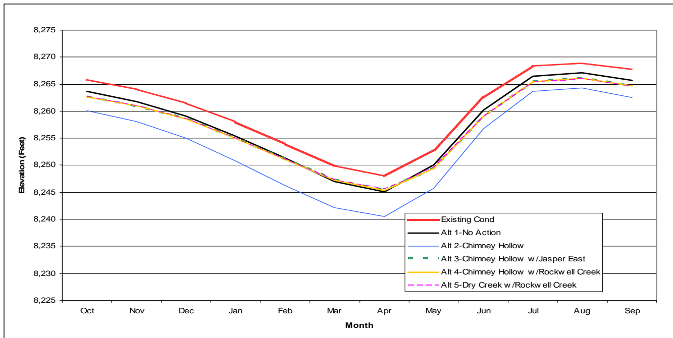
Figure 3-17. Granby Reservoir estimated average monthly surface elevation by alternative.
