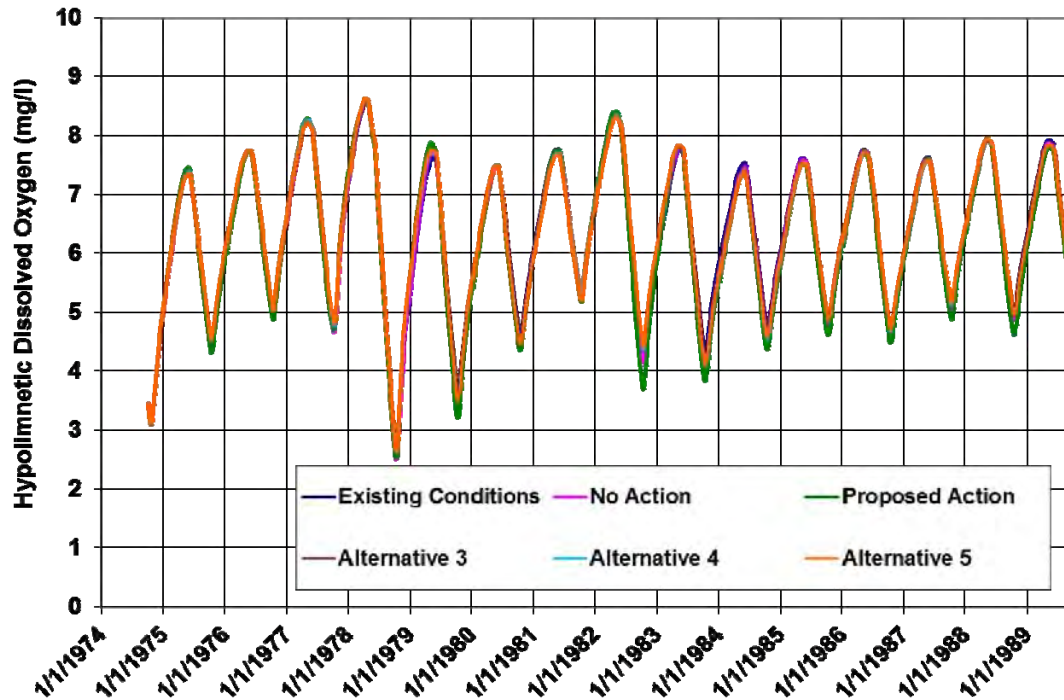
Figure 3-72. Simulated daily hypolimnetic dissolved oxygen in Granby Reservoir (existing conditions and all alternatives).
