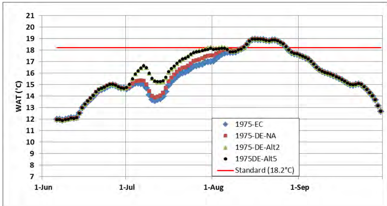
Figure 3-48. WAT at Colorado River downstream of Windy Gap Reservoir (WGD), June to September 1975.
