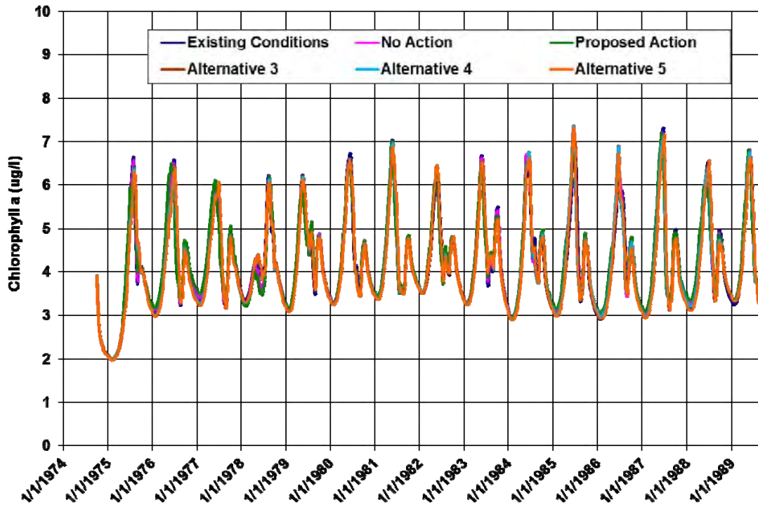
Figure 3-70. Simulated daily chlorophyll a concentrations in Granby Reservoir (existing conditions and all alternatives).
