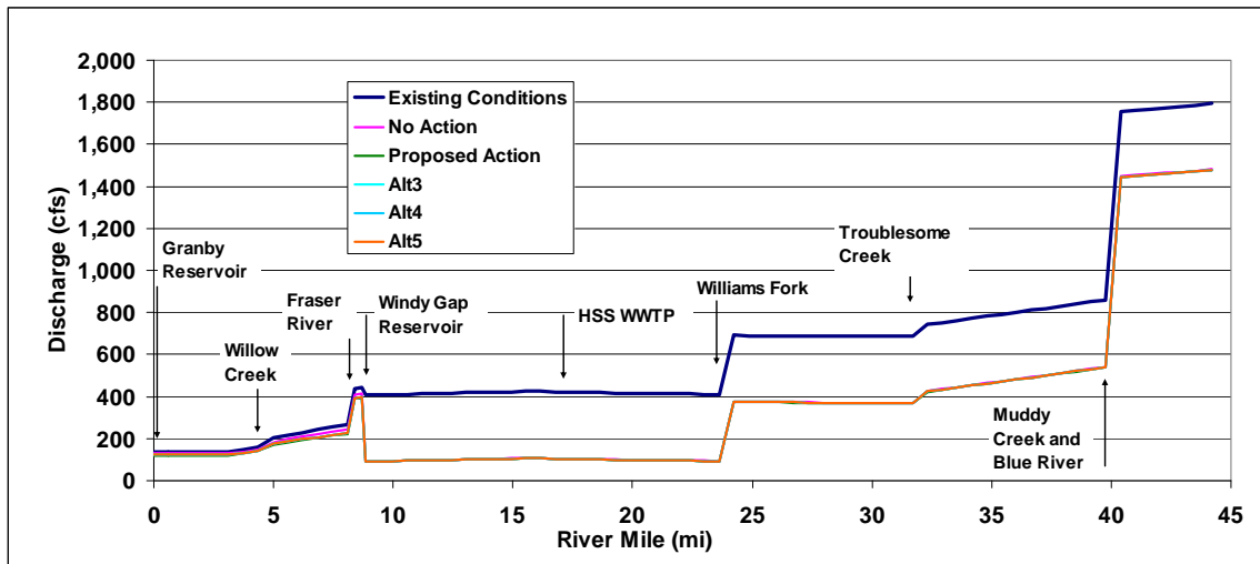
Figure 3-55. Colorado River July 25 streamflow assuming diversion to the minimum instream flow below Windy Gap Reservoir.
