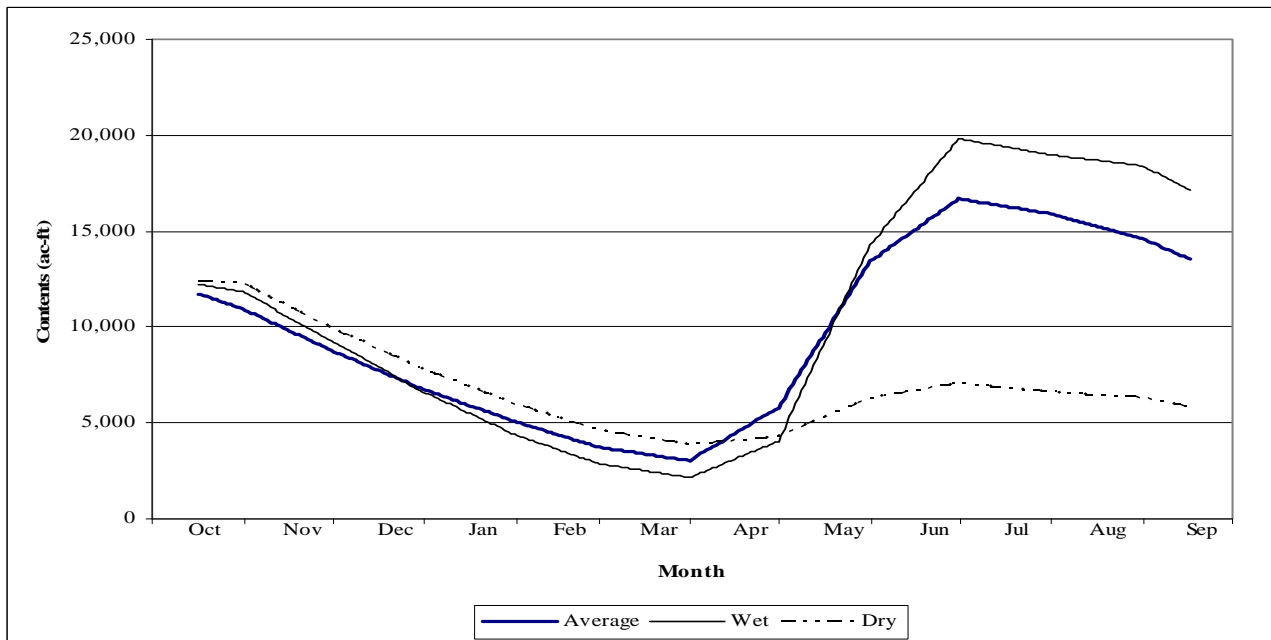
Figure 3-23. Jasper East Reservoir daily content under Alternative 3.
