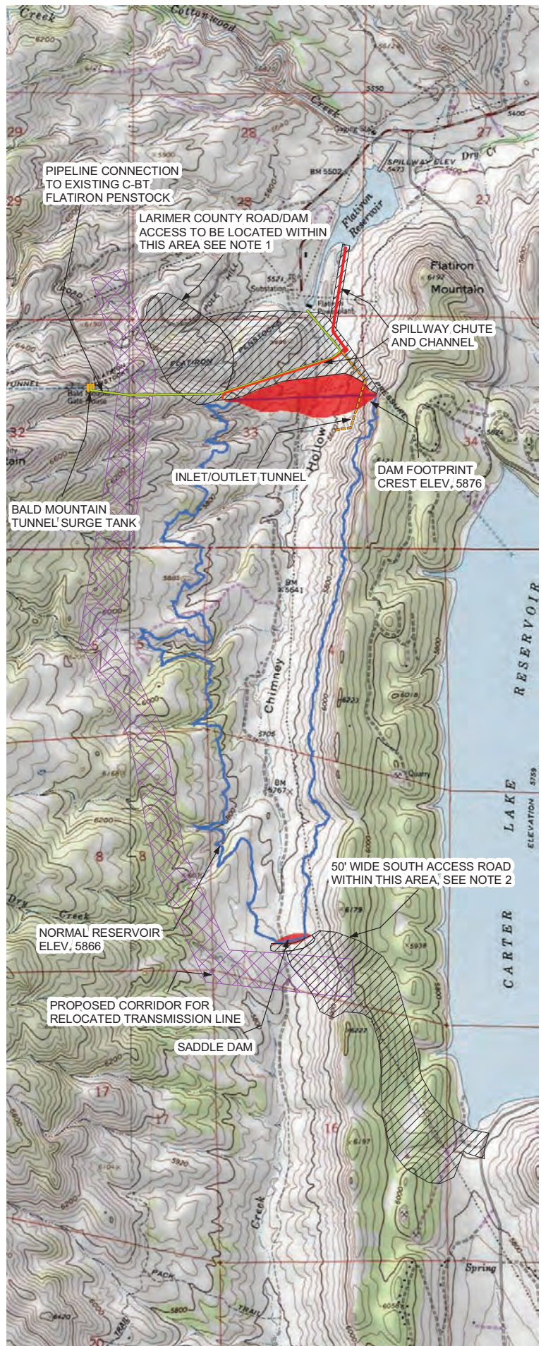
Figure 2-5 Alternative 2, Proposed Action Chimney Hollow Reservoir (90,000 AF)
