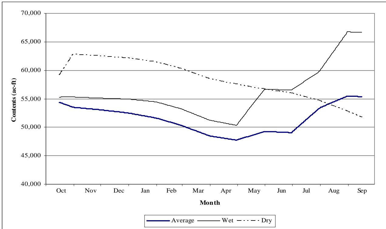
Figure 3-22. Chimney Hollow Reservoir daily content under Alternatives 3 and 4.
