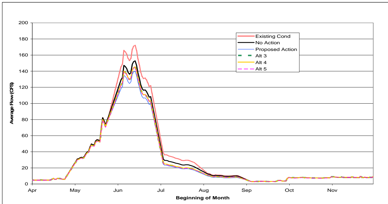
Figure 3-16. Willow Creek at Colorado River – average daily flows by alternative.
