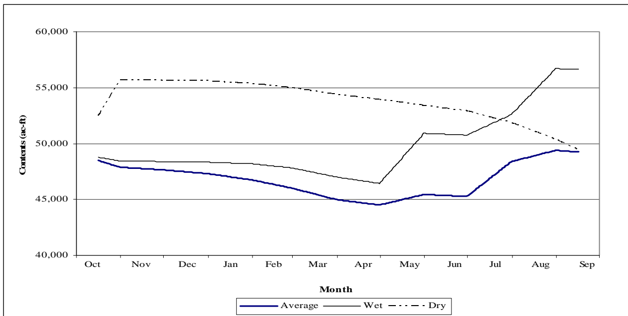
Figure 3-24. Dry Creek Reservoir daily content under Alternative 5.
