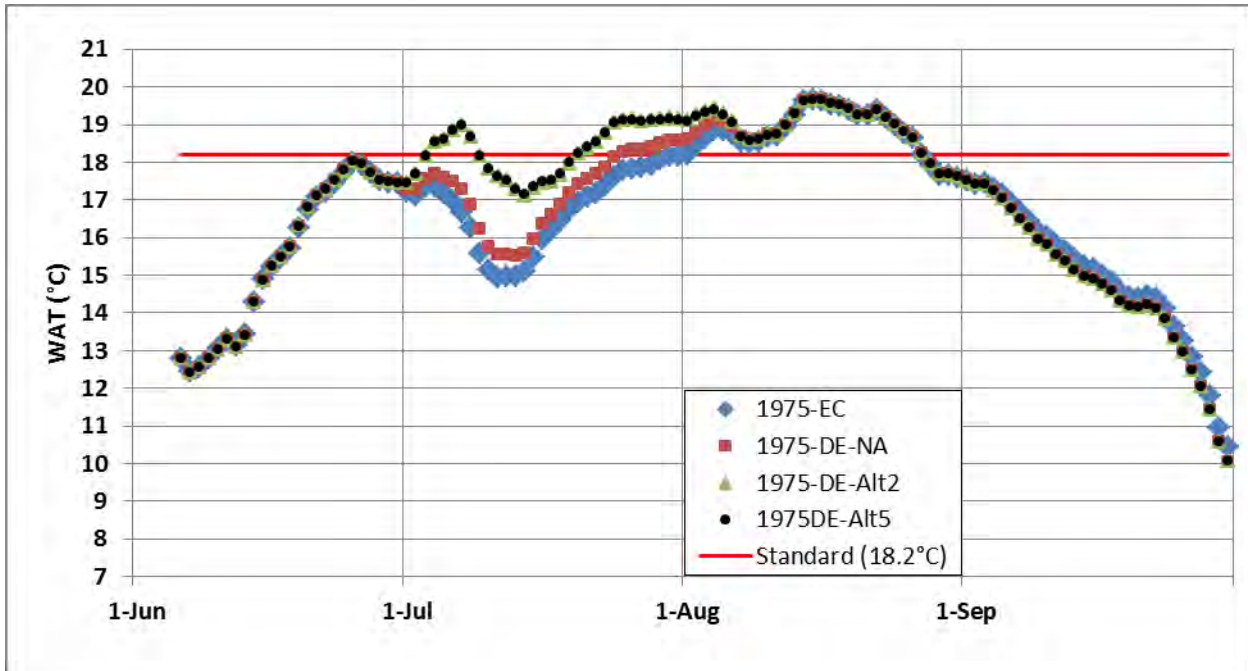
Figure 3-50. WAT at Colorado River upstream of the Williams Fork (WFU), June to September 1975.
