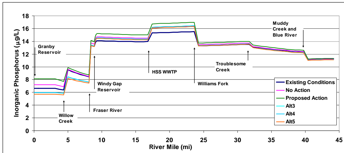
Figure 3-62. Colorado River inorganic phosphorus concentrations for July 25.
