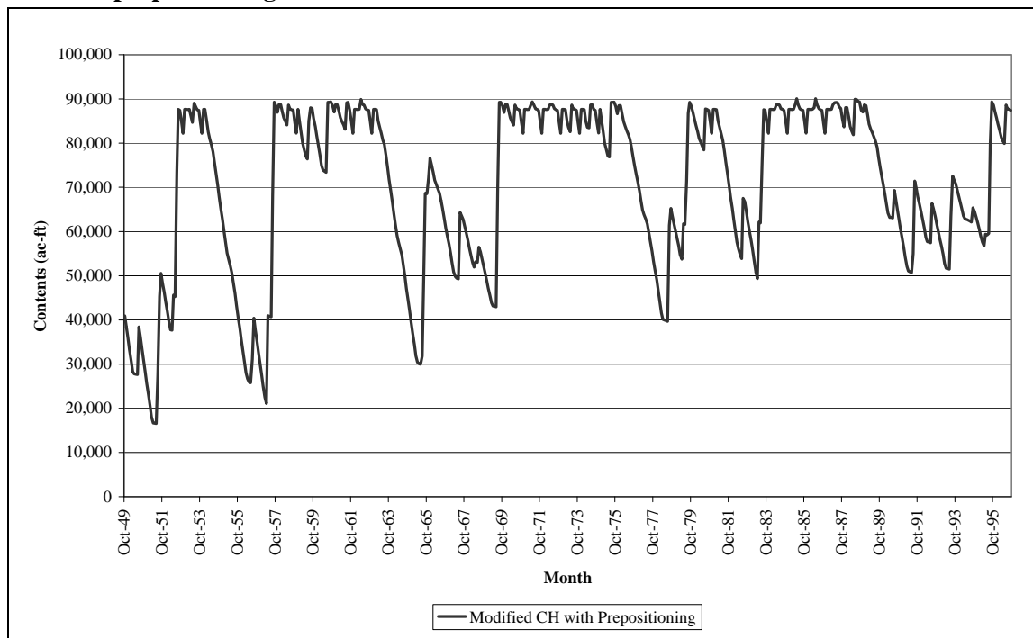
Figure 3-30. Chimney Hollow Reservoir operation for the Proposed Action with modified prepositioning.
