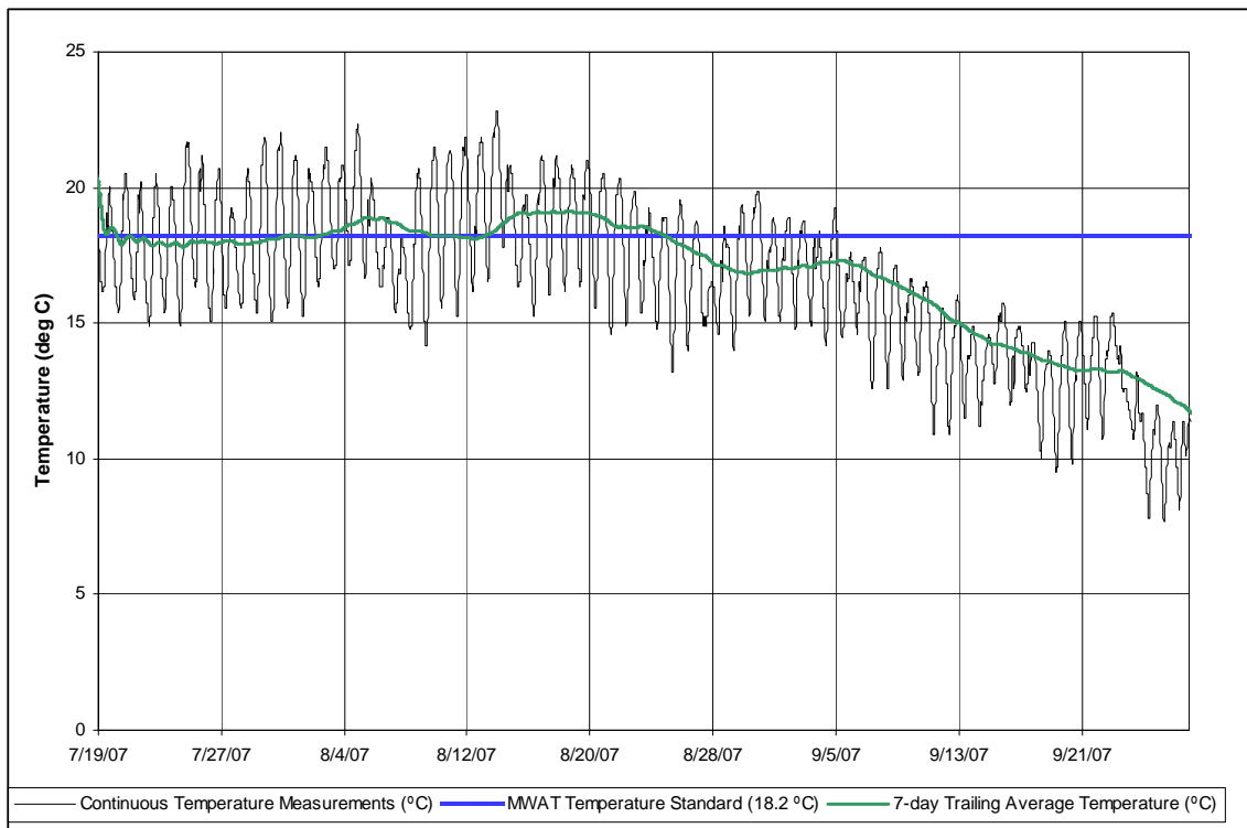
Figure 3-38. Colorado River temperatures at Lone Buck in 2007.
