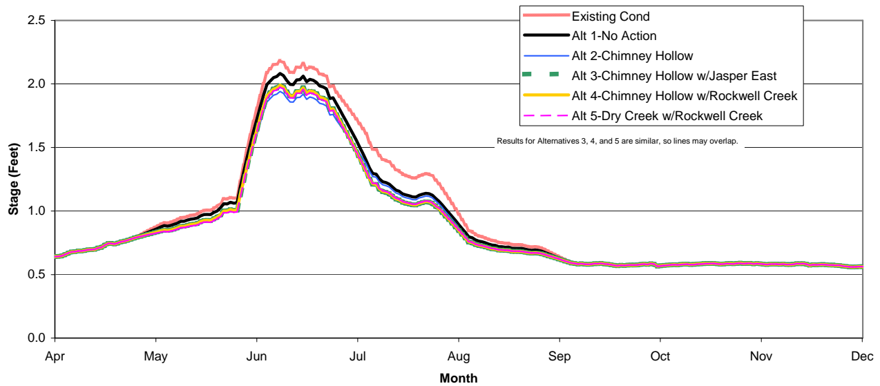
Figure 3-108. Colorado River stream stage at Hot Sulphur Springs.
