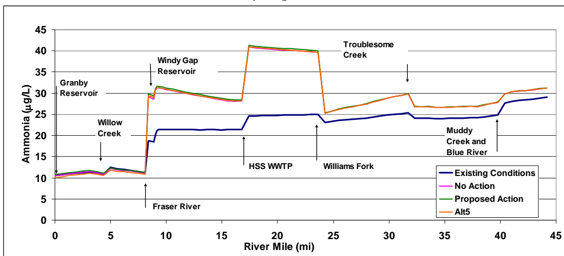
Figure 3-86. Colorado River ammonia concentrations for July 25 assuming diversion to the minimum streamflow below Windy Gap Reservoir—cumulative effects.
