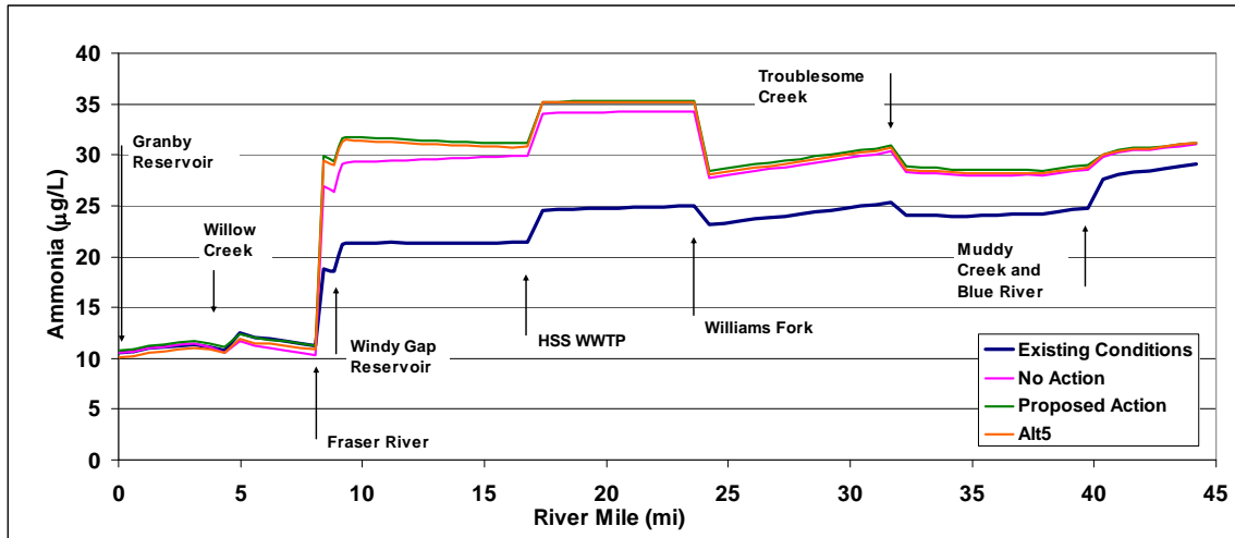
Figure 3-85. Colorado River ammonia concentrations for July 25—cumulative effects.
