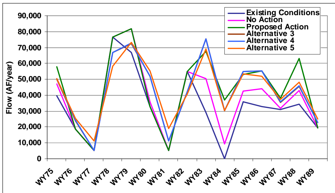
Figure 3-64. Estimated pumping from Windy Gap Reservoir, proposed Jasper East Reservoir (Alternative 3), and proposed Rockwell Creek Reservoir (Alternatives 4 and 5) into Granby Reservoir by water year.
