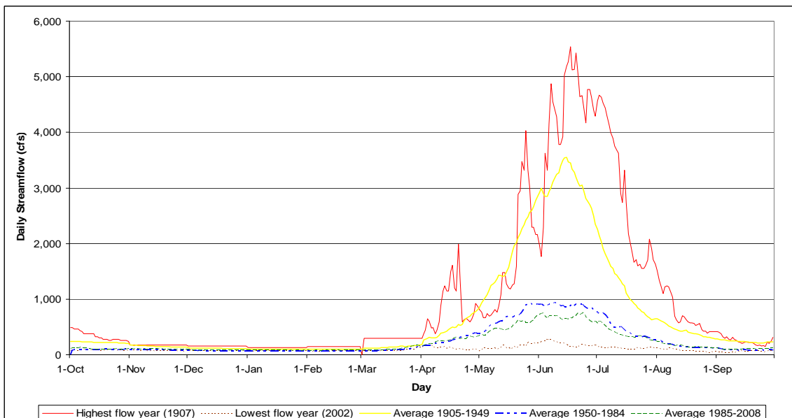
Figure 3-4. Colorado River average daily flow at Hot Sulphur Springs and Windy Gap, 1904 to 2008.
