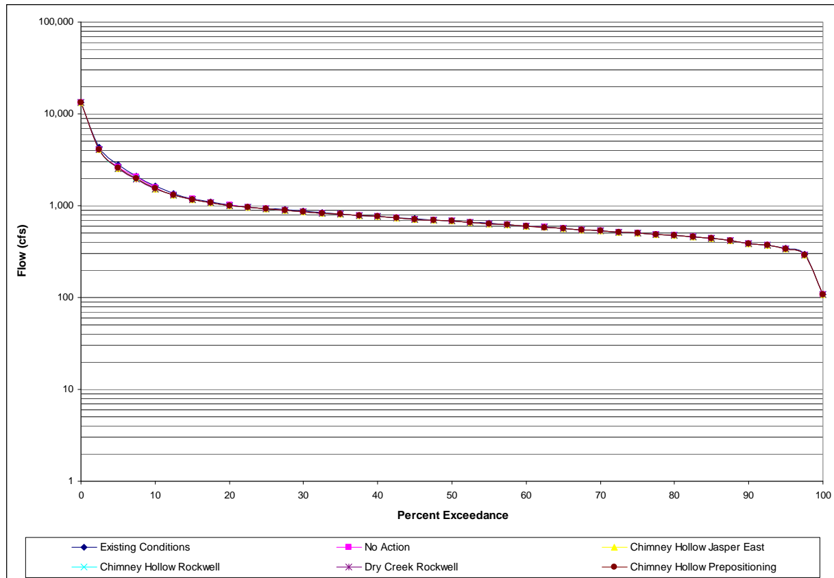
Figure 3-33. Flow duration curve—Colorado River at Kremmling below Blue River.
