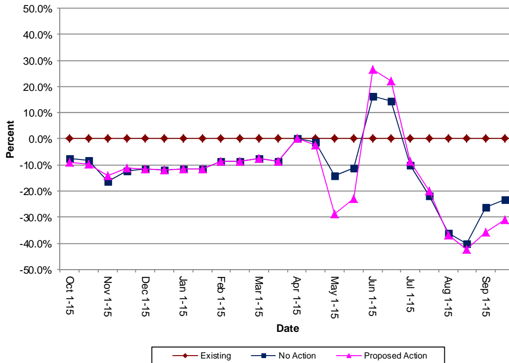
Figure 3-104. Percent change in rainbow trout (adult) habitat from existing conditions on the Colorado River below Windy Gap for average water year, cumulative effects.
