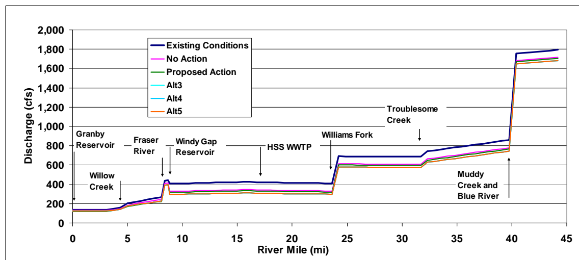
Figure 3-54. Colorado River average July 25 streamflow.
