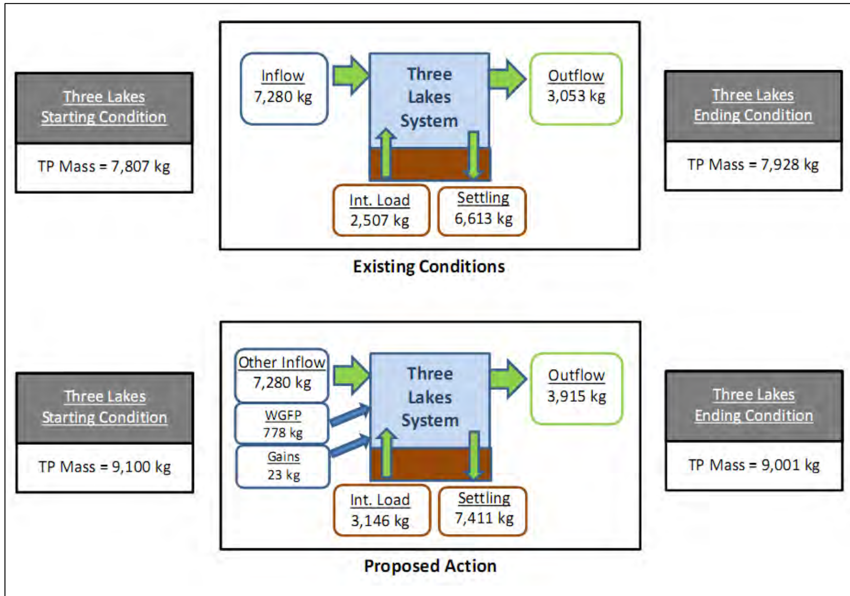
Figure 3-66. Fate of total phosphorus (TP) for the Three Lakes system (average annual kg/yr, WY75-WY89).
