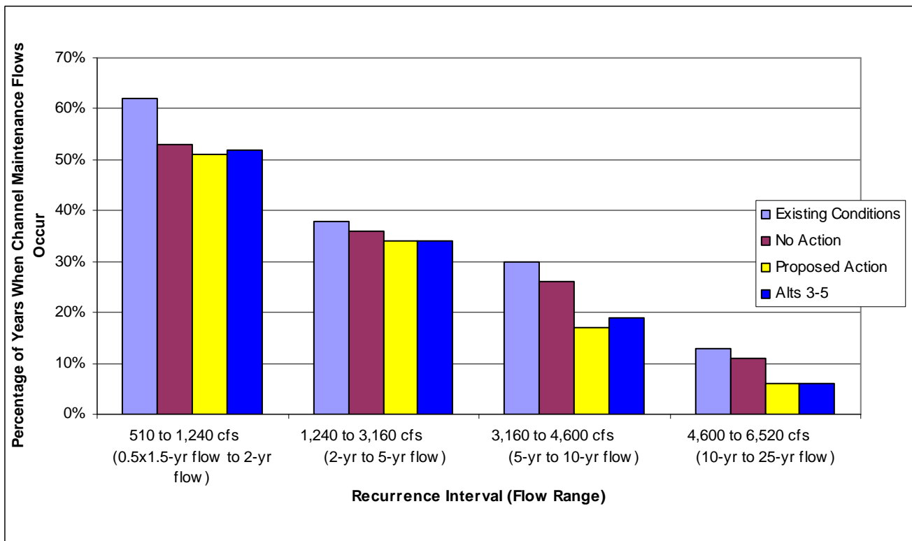
Figure 3-35. Percent of years when channel maintenance flows occur at Hot Sulphur Springs.
