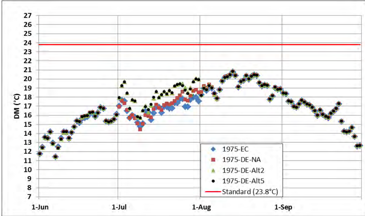
Figure 3-51. Daily Maximum Temperature at Colorado River downstream of Windy Gap Reservoir (WGD), June to September 1975.
