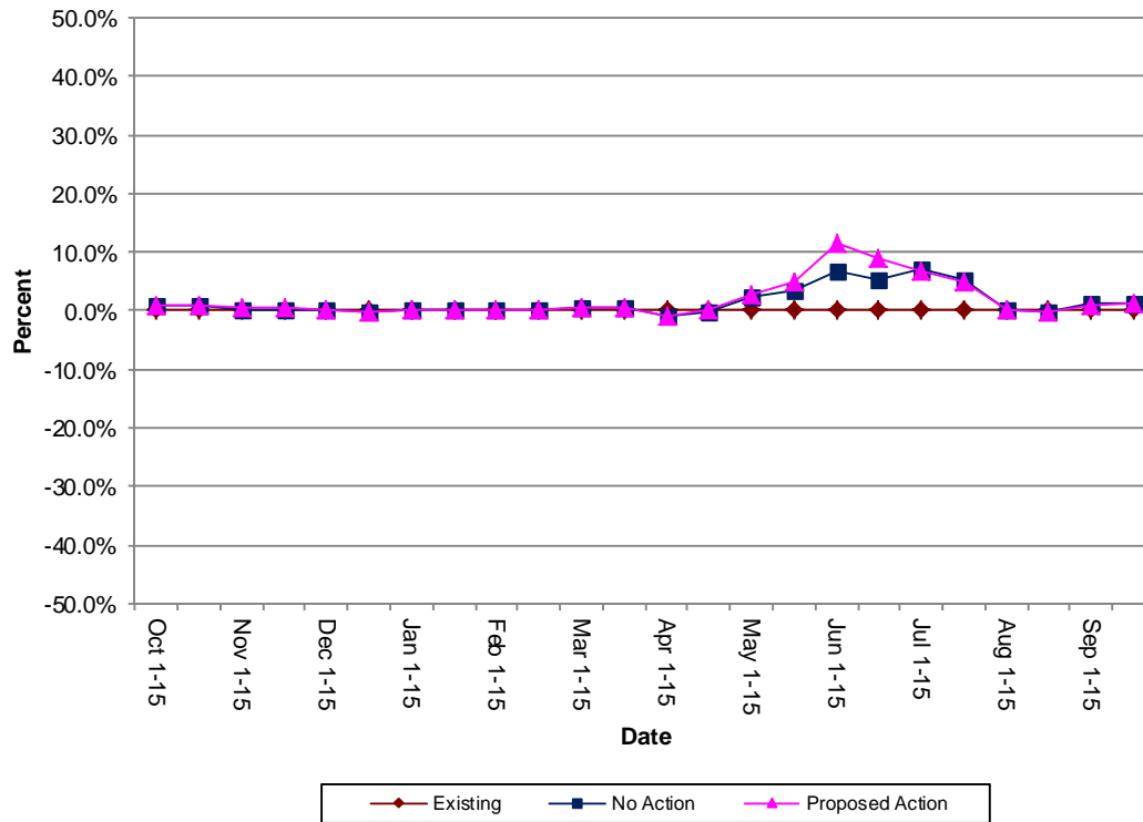
Figure 3-107. Percent change in brown trout (adult) habitat from existing conditions on the Colorado River above the Blue River for average water year, cumulative effects.
