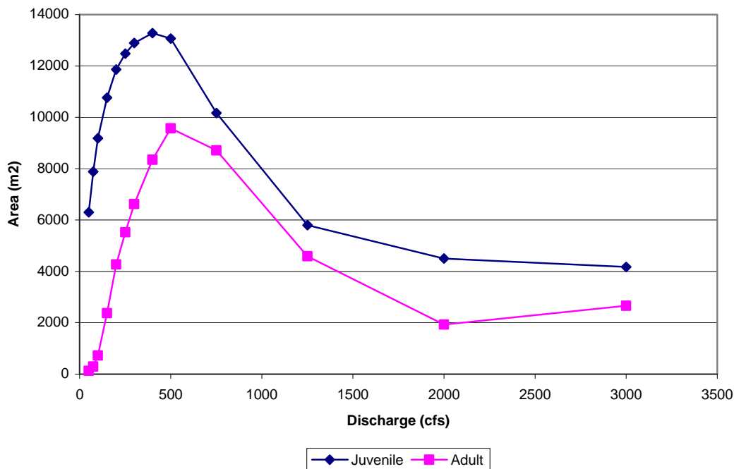
Figure 3-94. Rainbow trout habitat area versus discharge – Lone Buck site, Colorado River.
