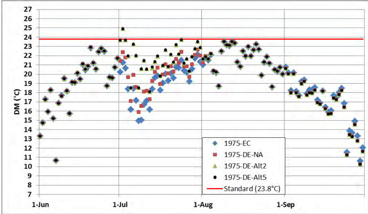
Figure 3-53. Daily Maximum Temperature at Colorado River upstream of the Williams Fork (WFU), June to September 1975.
