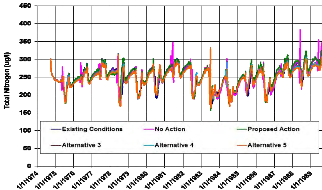
Figure 3-79. Simulated daily total nitrogen concentrations in Grand Lake (existing conditions and all alternatives).
