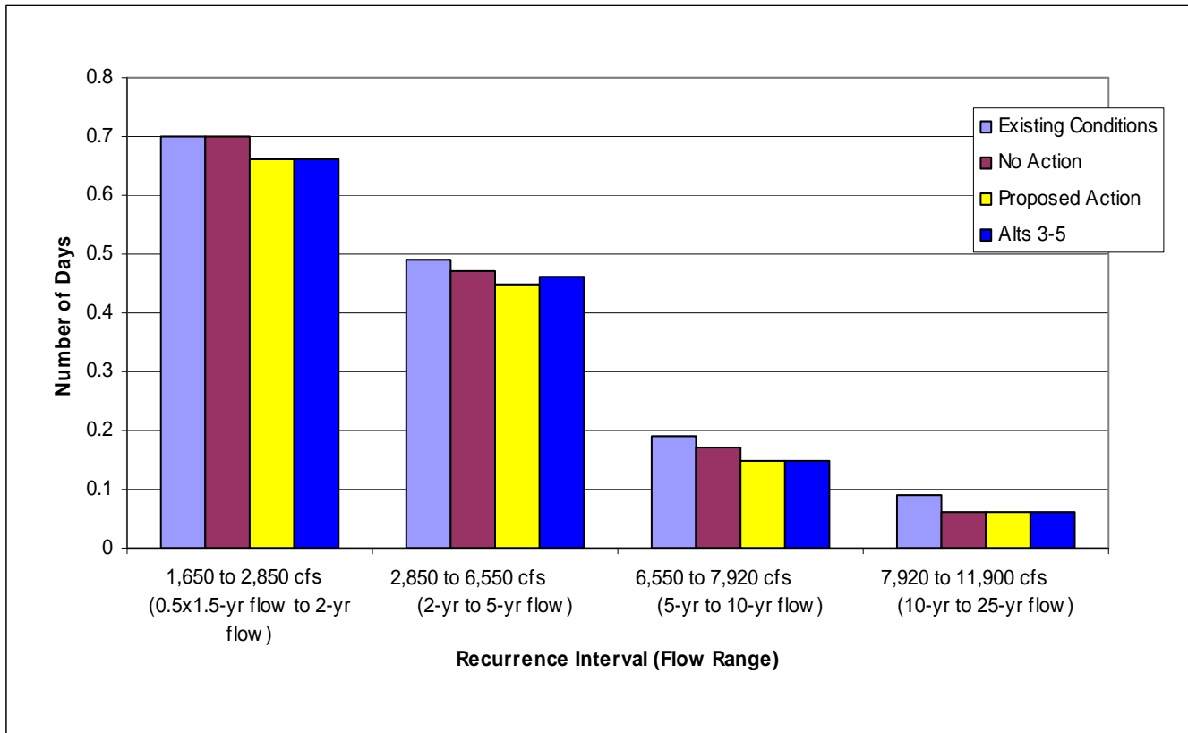
Figure 3-37. Percent of years when channel maintenance flows occur near Kremmling.
