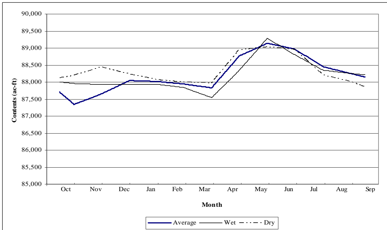
Figure 3-21. Chimney Hollow Reservoir daily content under the Proposed Action.
