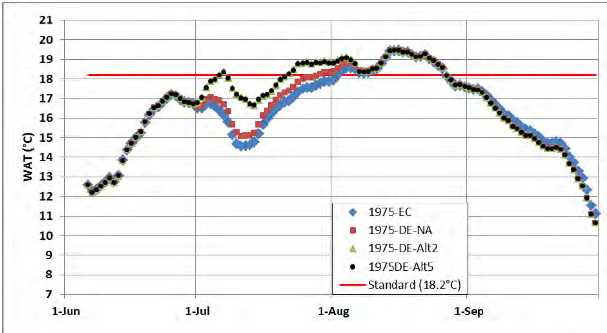
Figure 3-49. WAT at Colorado River at Hot Sulphur Springs (HSU), June to September 1975.
