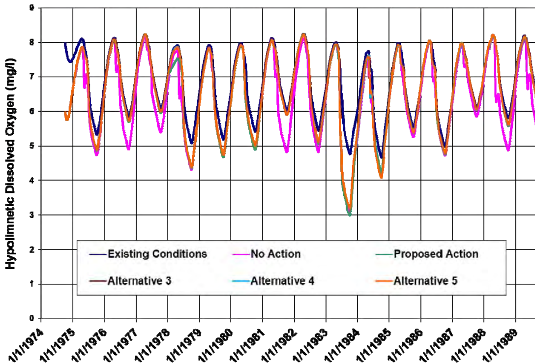
Figure 3-82. Simulated daily hypolimnetic dissolved oxygen in Grand Lake (existing conditions and all alternatives).
