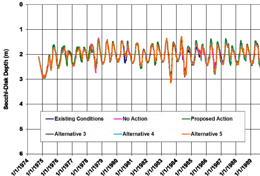
Figure 3-76. Simulated daily Secchi depth in Shadow Mountain Reservoir (existing conditions and all alternatives).
