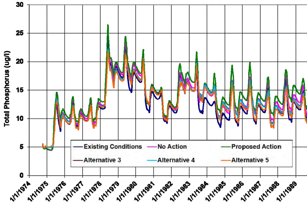
Figure 3-68. Simulated daily total phosphorus concentrations in Granby Reservoir (existing conditions and all alternatives).
