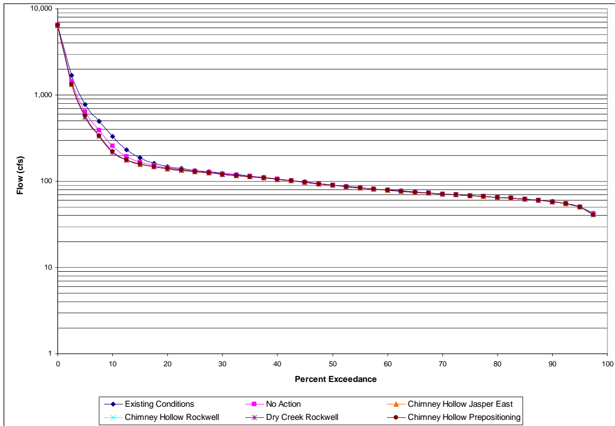
Figure 3-32. Flow duration curve—Colorado River at Hot Sulphur Springs.
