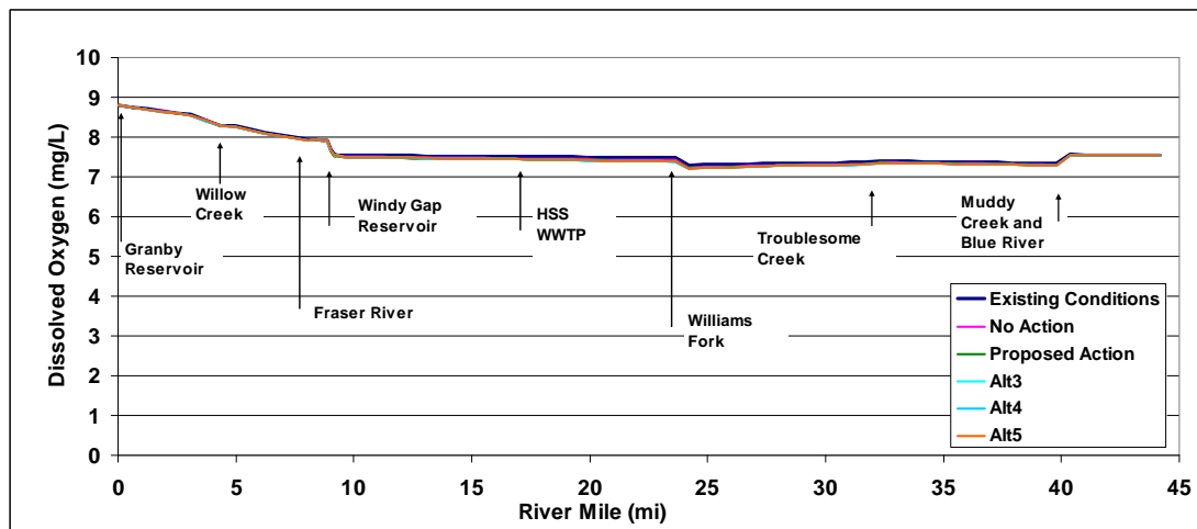
Figure 3-58. Colorado River dissolved oxygen concentrations for July 25.
