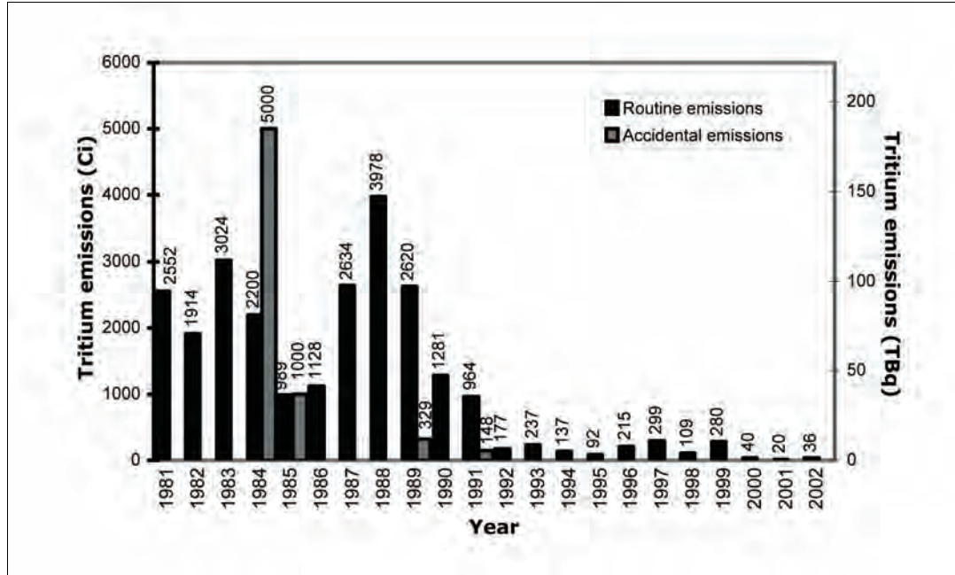
FIGURE 4.10.5–1.—Tritium Emissions From the Tritium Facility, 1981-2002
