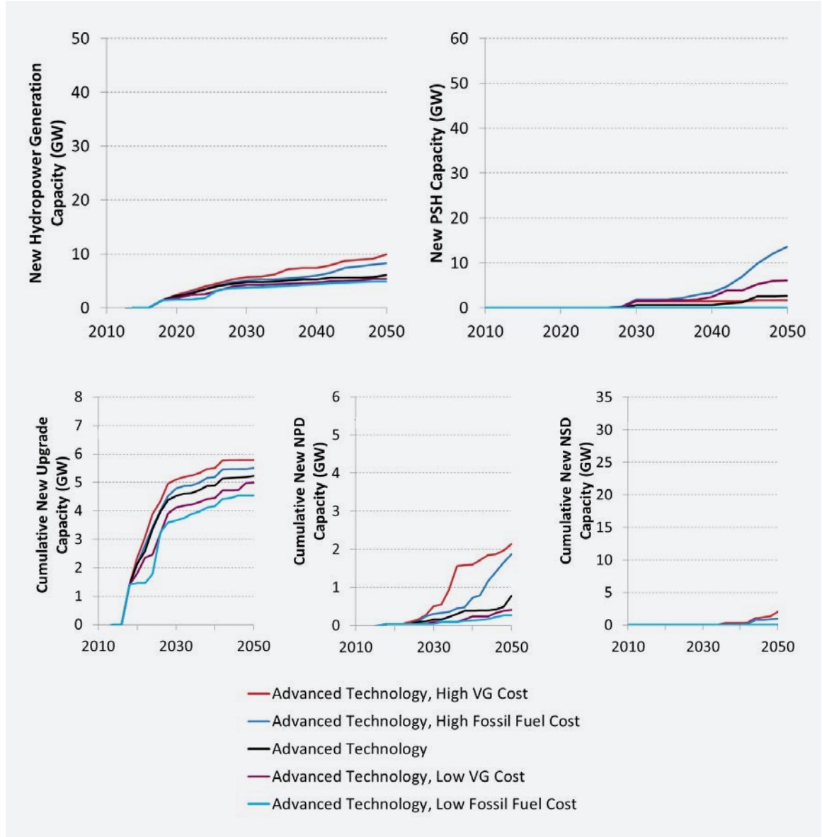
Figure F-9. Cumulative post-2016 capacity growth of total hydropower generation, PSH, and each category of hydropower generation (upgrades, NPD, and NSD) in fossil fuel and VG cost scenarios with Advanced Technology assumptions (note: each panel uses a unique y-axis)
