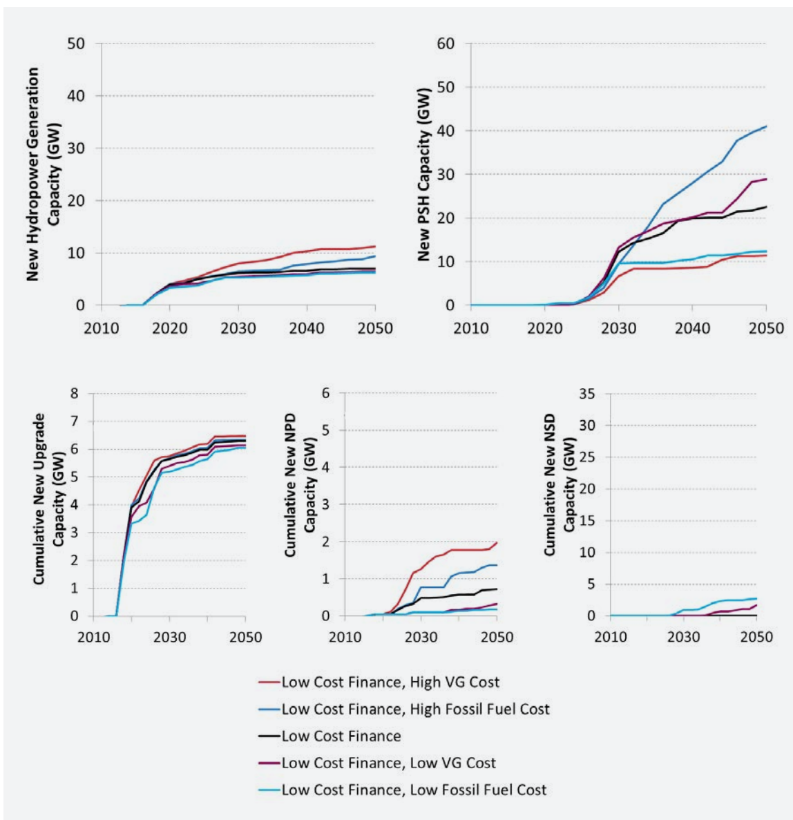
Figure F-10. Cumulative post-2016 capacity growth of total hydropower generation, PSH, and each category of hydropower generation (upgrades, NPD, and NSD) in fossil fuel and VG cost scenarios with Low Cost Finance assumptions (note: each panel uses a unique y-axis)
