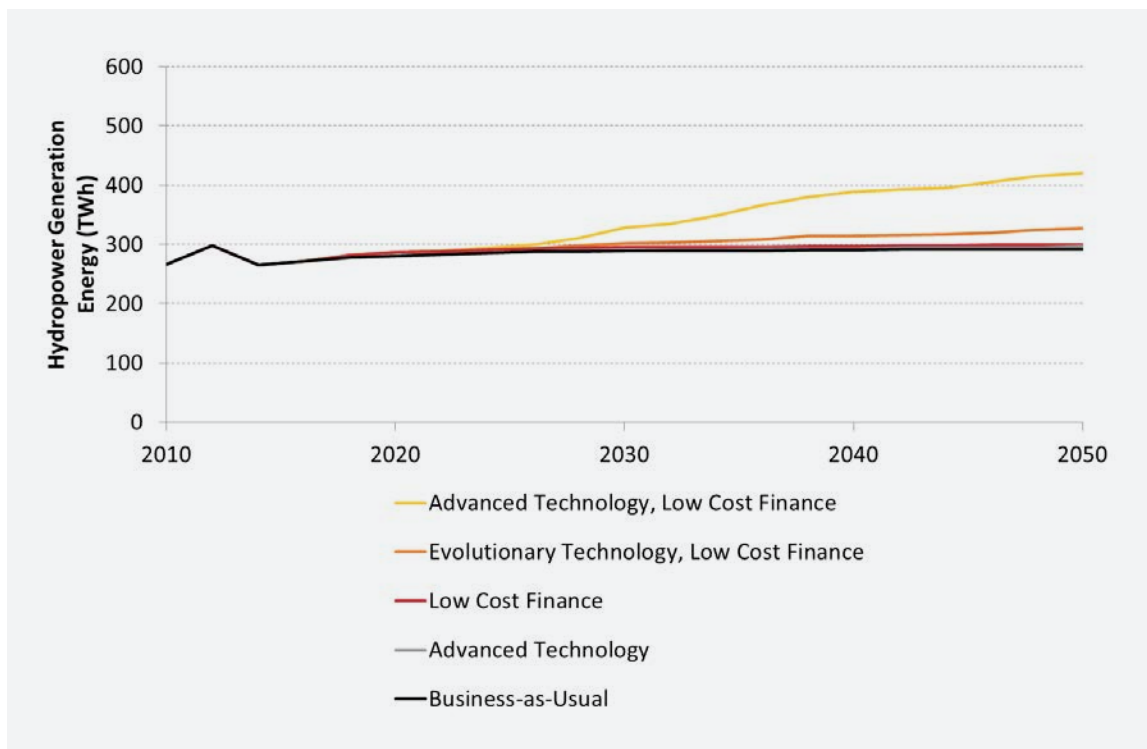
Figure F-14. Electricity generation from the existing hydropower fleet and growth in upgrades, NPD, and NSD (excludes net generation from PSH) in hydropower technology cost scenarios
