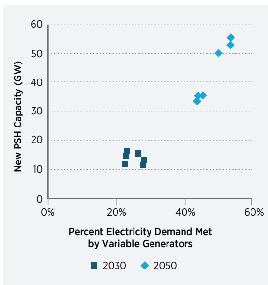
Figure 3-17. The relationship between new pumped storage hydropower growth and generation from variable generators for fuel and cost sensitivities under Advanced Technology and Low Cost Finance conditions
