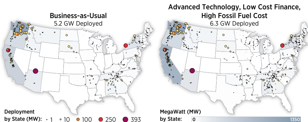
Figure 3-19. Regional deployment of upgrades for representative low and high deployment
