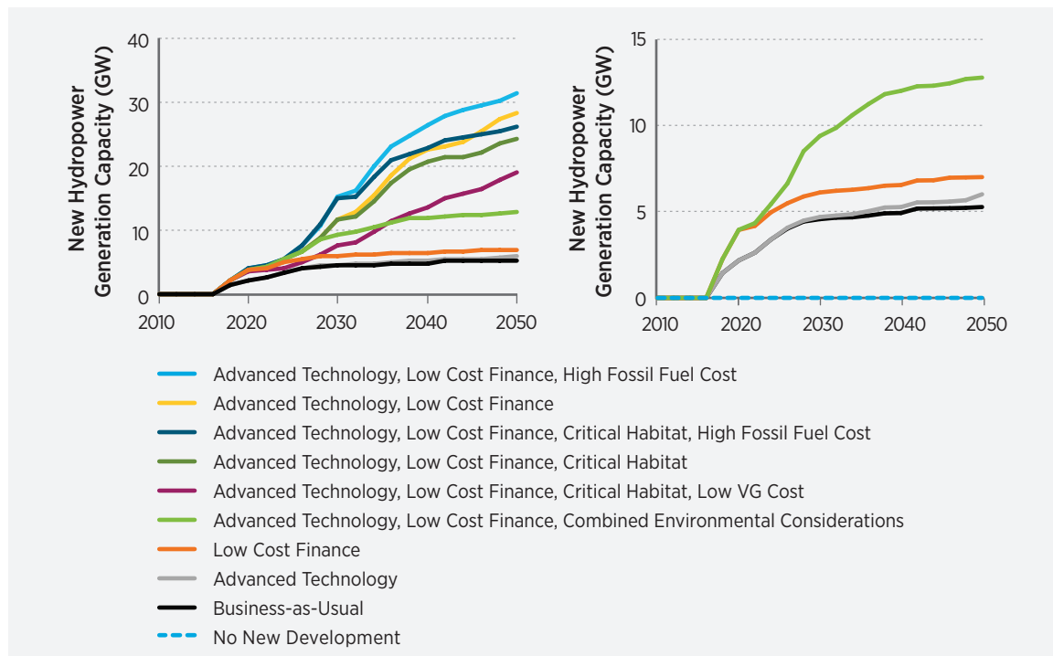
Figure O3-2. ReEDS modeled deployment of new hydropower generation capacity (GW) in 2017-2050 for the nine selected scenarios (left panel) and the four scenarios highlighted in this overview (right panel) [each panel uses a unique y-axis]
