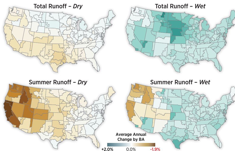
Figure 3-6. Average annual and summer seasonal change in total runoff
