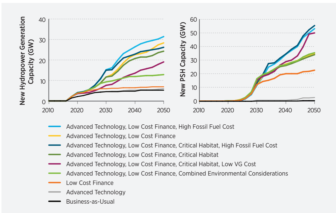
Figure 3-8. Capacity growth of hydropower generation and pumped storage hydropower in select deployment scenarios
