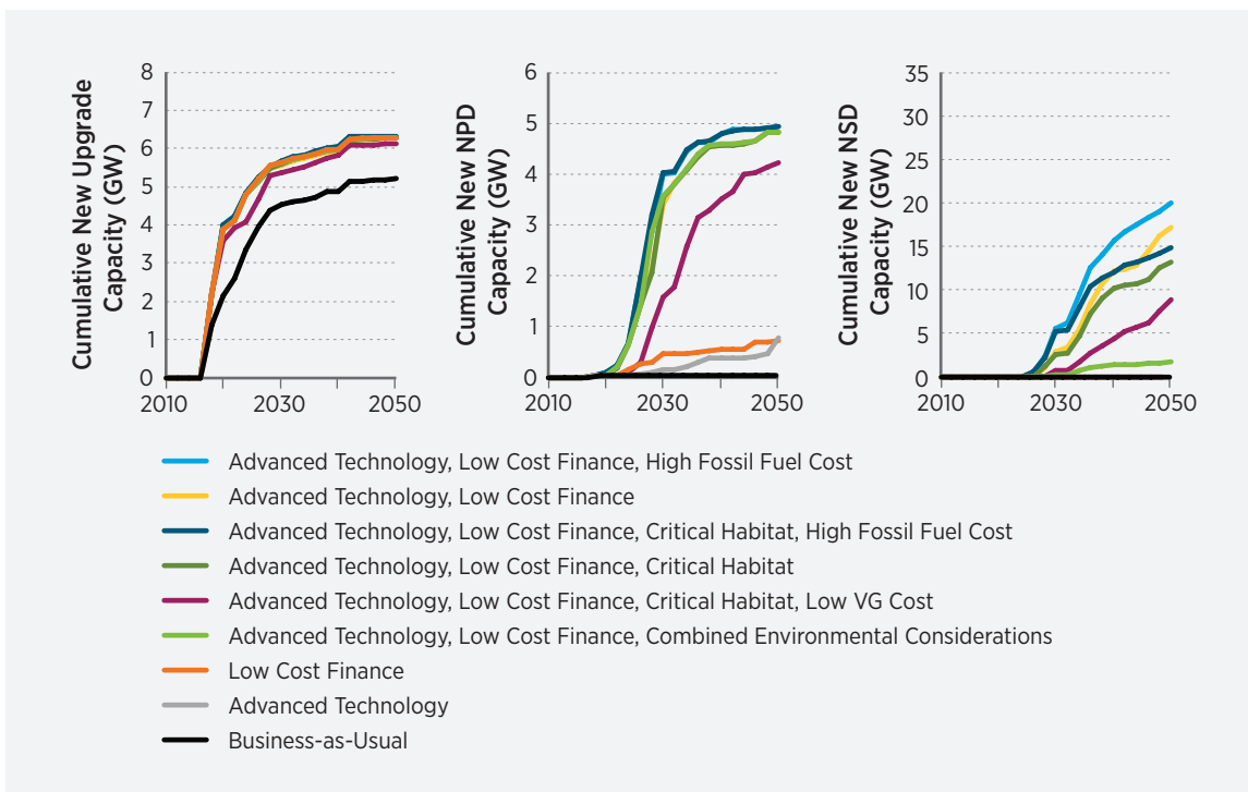
Figure 3-9. Capacity growth of upgrades, NPD, and NSD in select deployment scenarios (each panel uses a unique y-axis)
