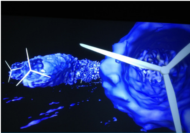
Immersive visualization of low-velocity wakes forming behind the turbines in an LES simulation of the Lilligrund wind farm. Image by Kenny Gruchalla, Nicholas Brunhart-Lupo & Matthew Churchfield, NREL
