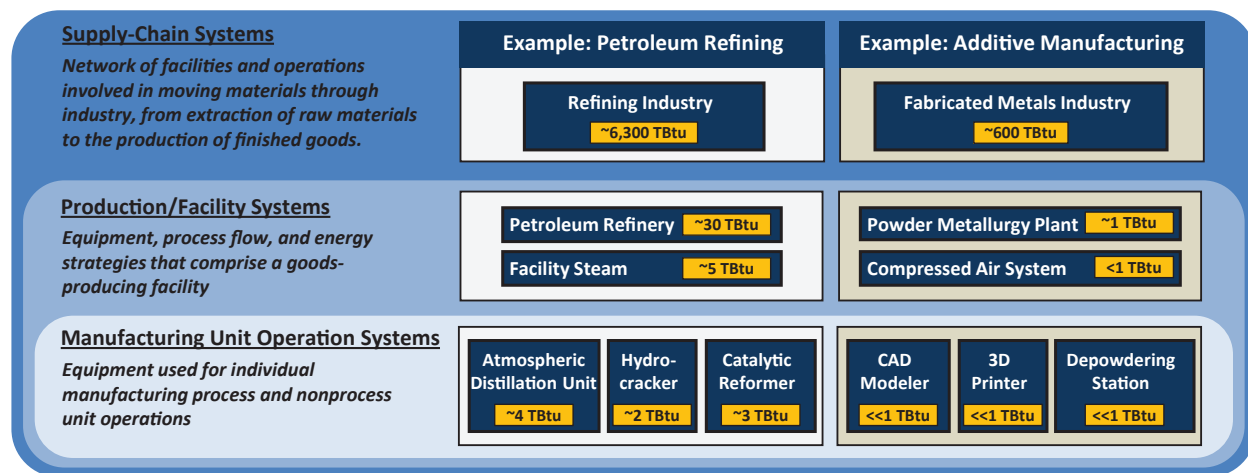
Figure 6.2 Levels of System Integration in Manufacturing. Opportunities for energy savings occur at each system level. The energy usage estimates shown (yellow boxes) represent the typical annual energy consumption levels in the United States for a single industry, production facility, or piece of manufacturing equipment.
