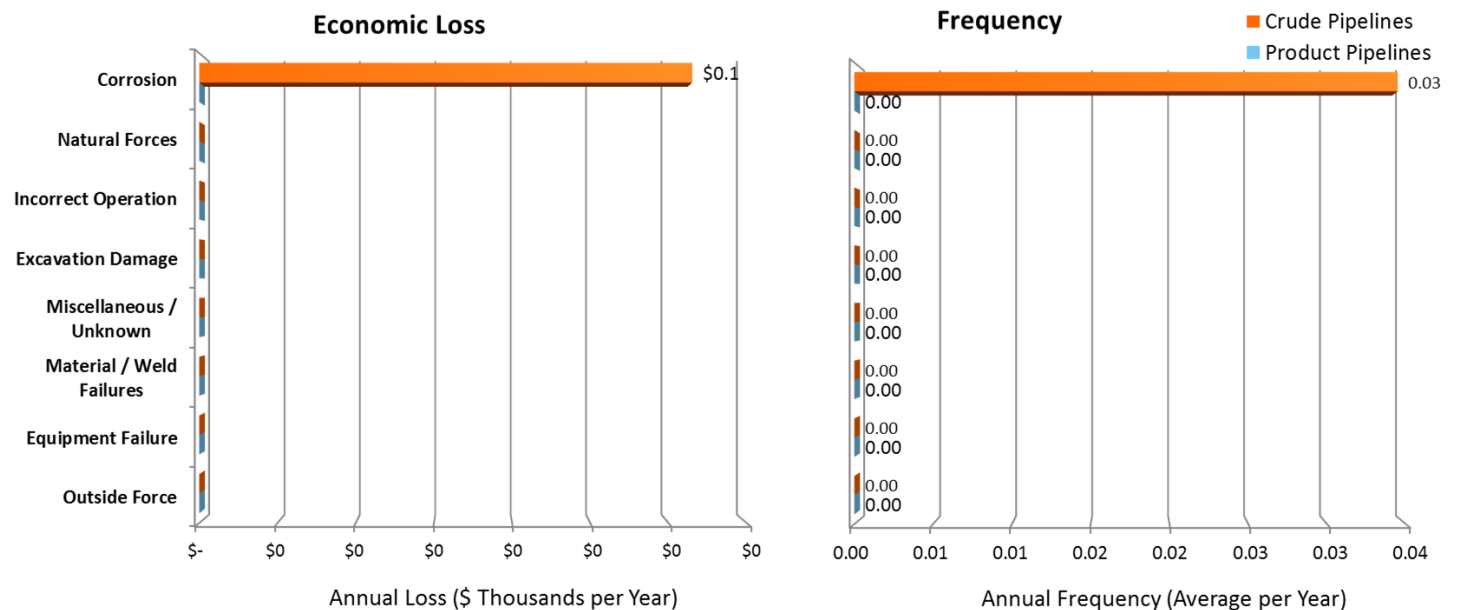
Top Events Affecting Crude Oil and Refined Product Pipelines in New Hampshire (1986–2014)
