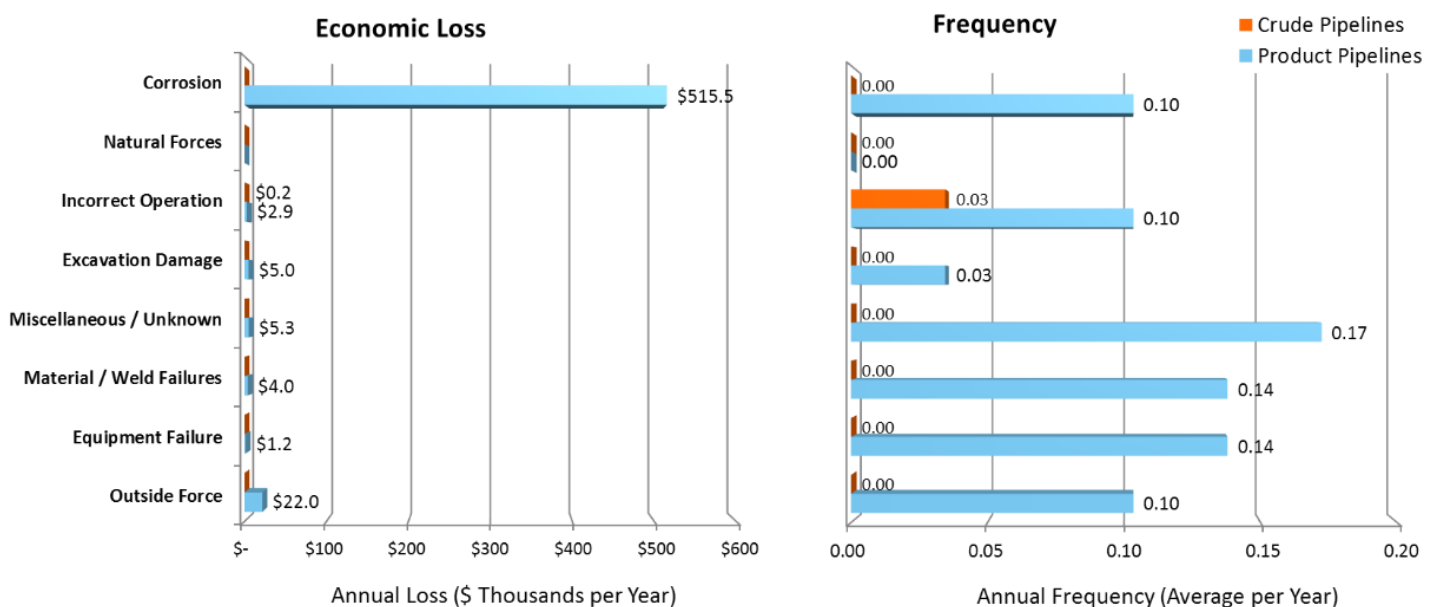
Top Events Affecting Crude Oil and Refined Product Pipelines in Arizona (1986–2014)
