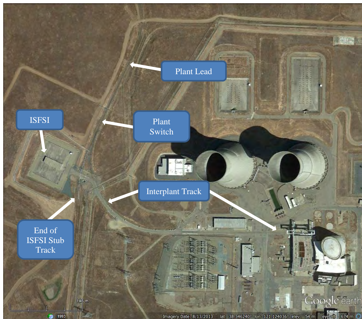
Figure B-10. Satellite View of the Rancho Seco Plant (Google 2013)
