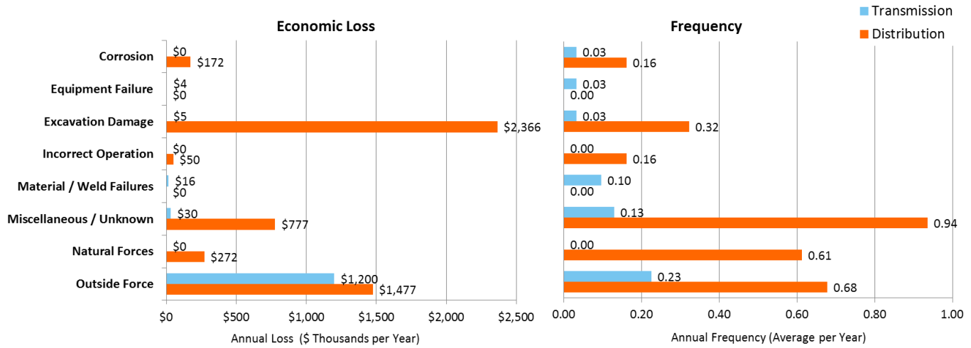
Top Events Affecting Natural Gas Transmission and Distribution in New Jersey (1986–2014)
