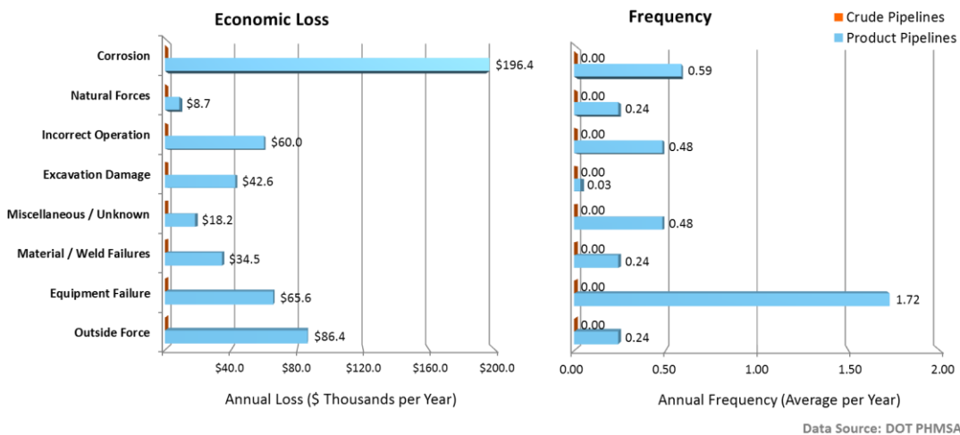
Top Events Affecting Crude Oil and Refined Product Pipelines in New Jersey (1986–2014)
