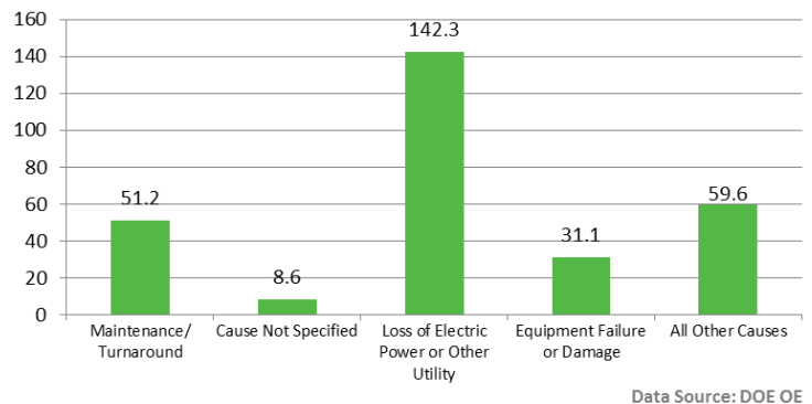
Average Production Impact (thousand barrels per day) from Petroleum Refinery Outages in Kentucky (2003–2014)
