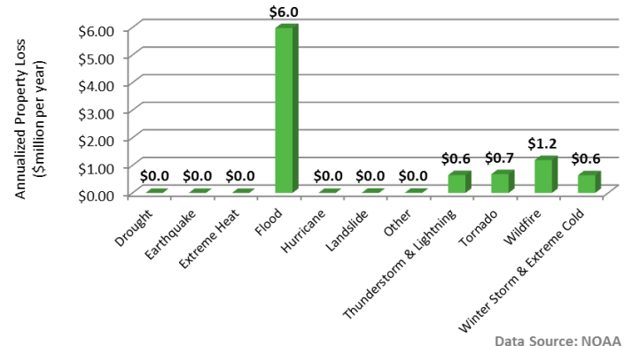
Annualized Property Loss due to Natural Hazards in Idaho (1996–2014)
