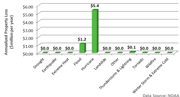
Annualized Property Loss due to Natural Hazards in Washington, D.C. (1996–2014)
