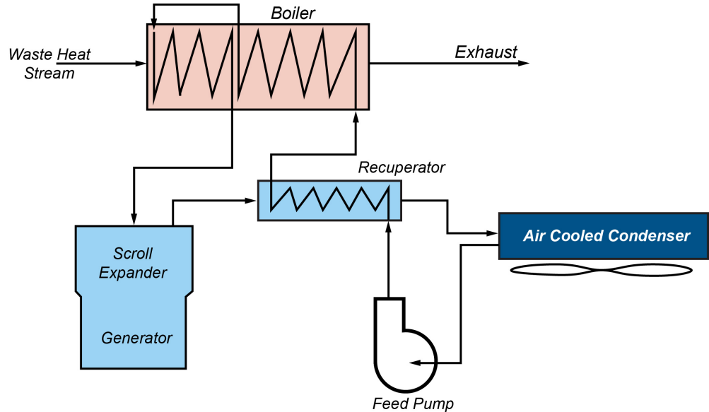
Bottoming cycle schematic with the scroll expander technology. Graphic credit TIAX.
