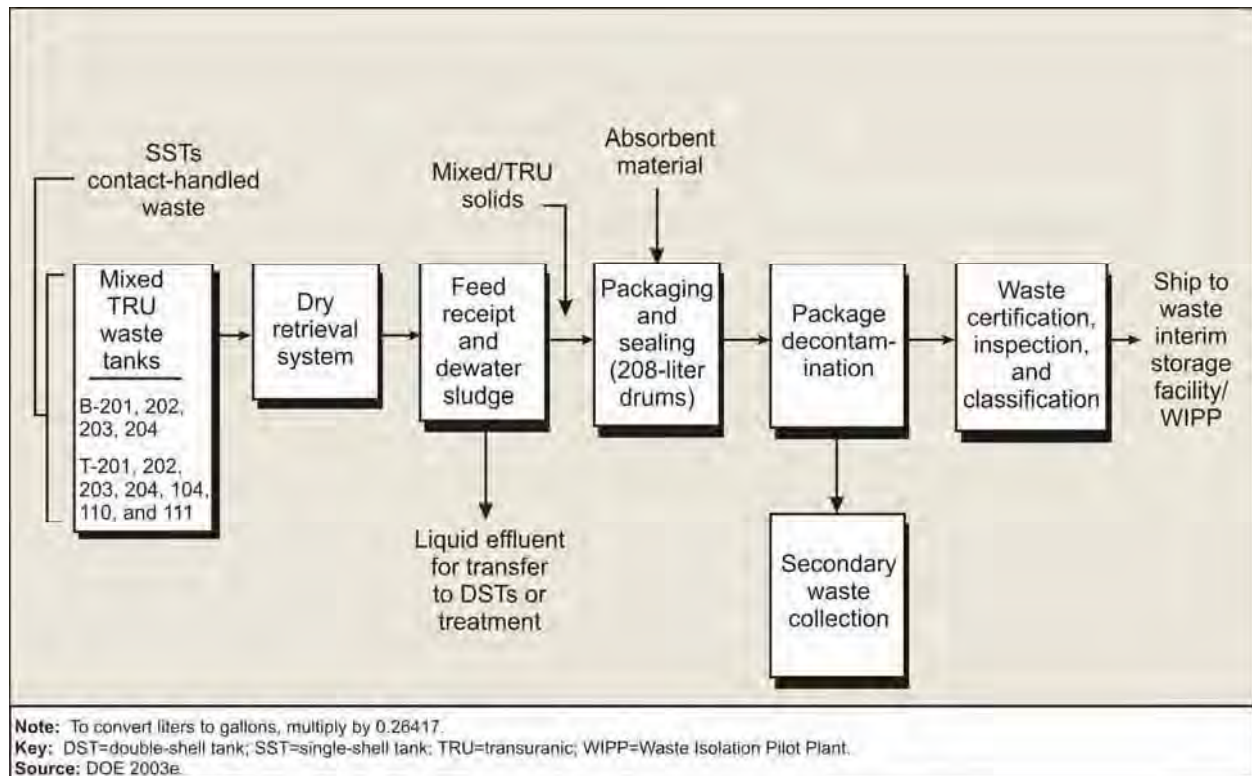
Figure E-23. Contact-Handled Mixed Transuranic Waste Packaging Process Flow Diagram
