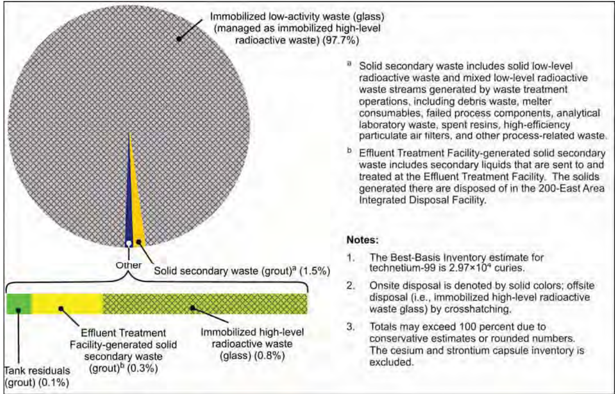
Figure D-57. Tank Closure Alternative 6B, Base Case or Option Case: Tchnetium-99 Distribution
