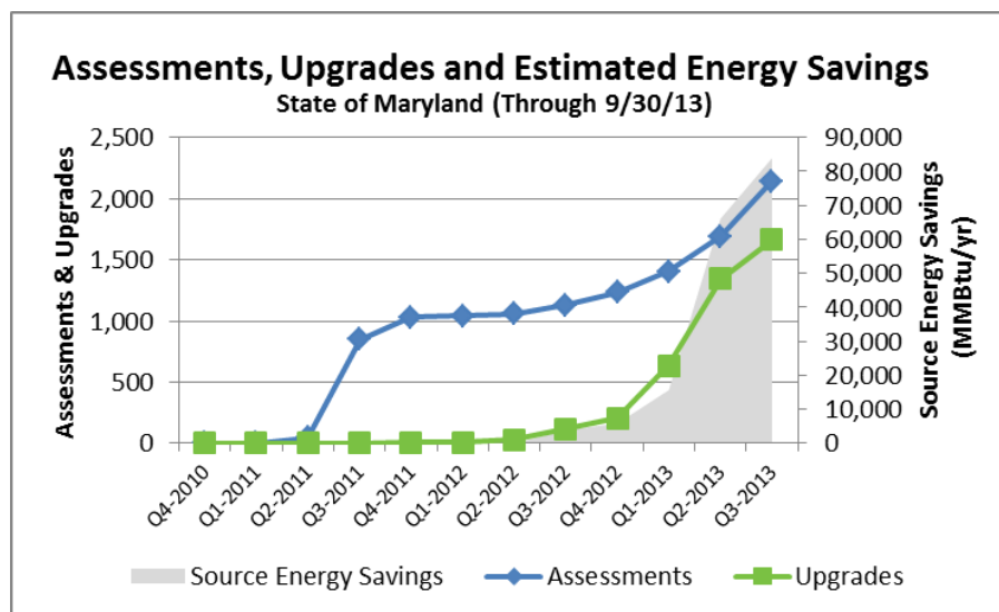
Figure 2. Maryland Assessments, Upgrades, and Estimated Savings
