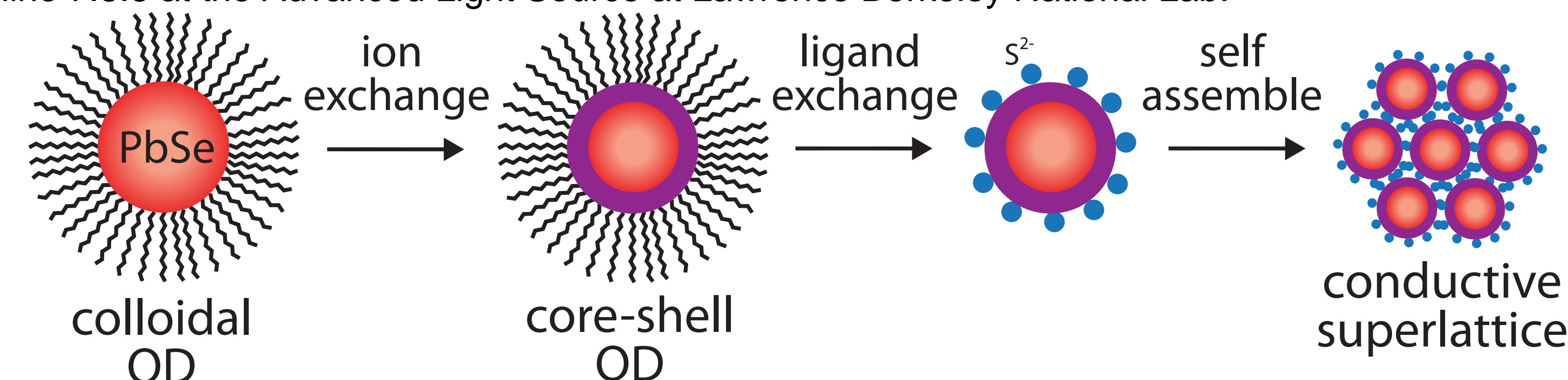
Scheme 1. Proposed process for forming conductive PbSe QD superlattice films. The TEM image shows a PbSe/CdSe core-shell QD made by ion exchange
