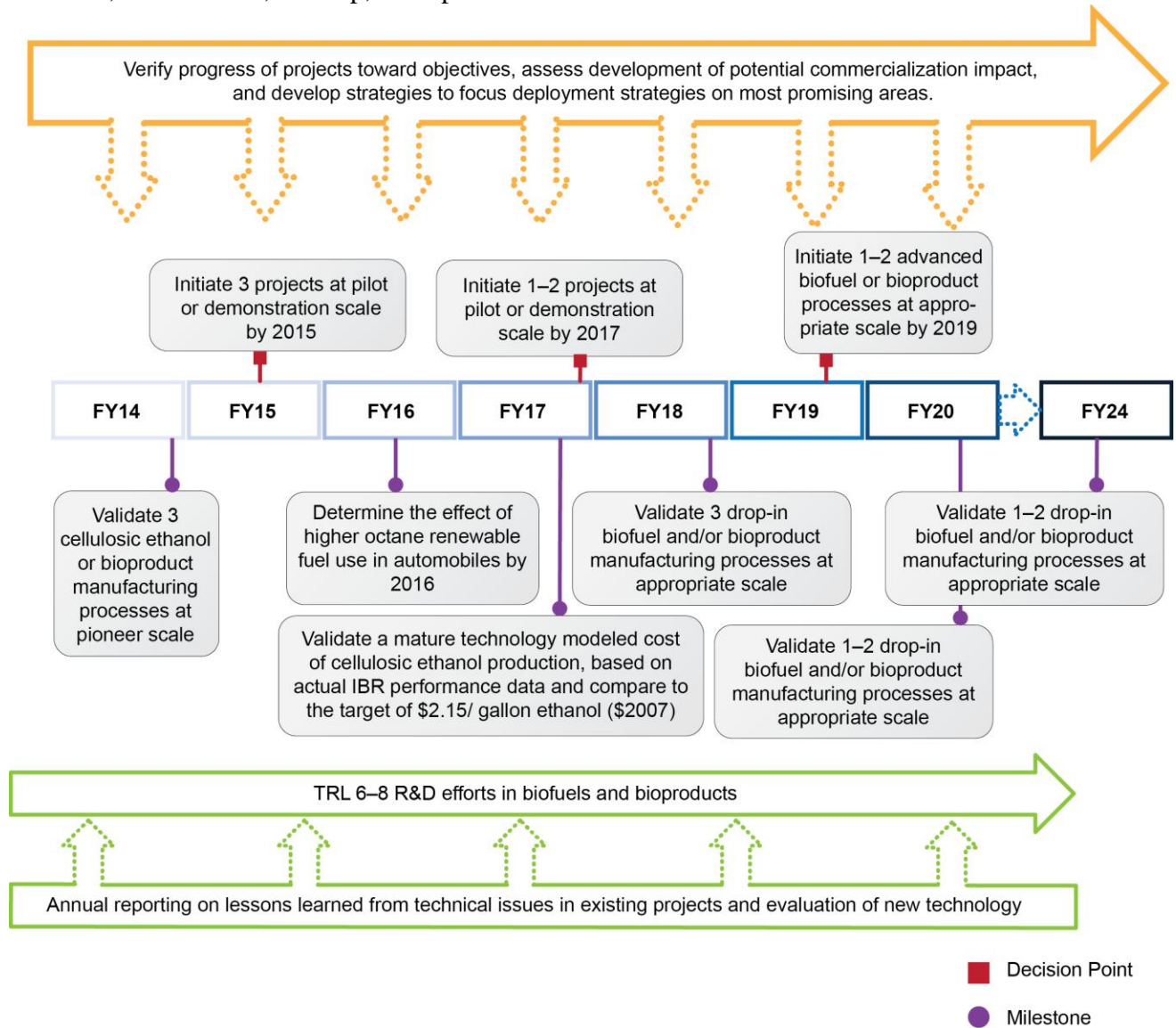
Figure 2-30: Demonstration and deployment key milestones and decision points
