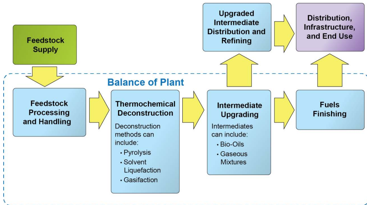
Figure 2-21: Thermochemical conversion process steps for biomass to biofuels
