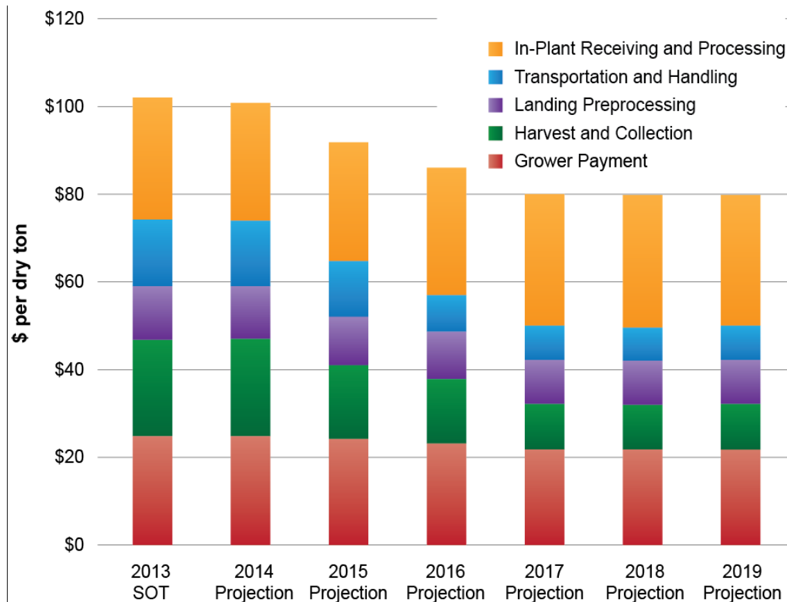
Figure 2-10: Historical and projected delivered feedstock costs, modeled for pyrolysis conversion
