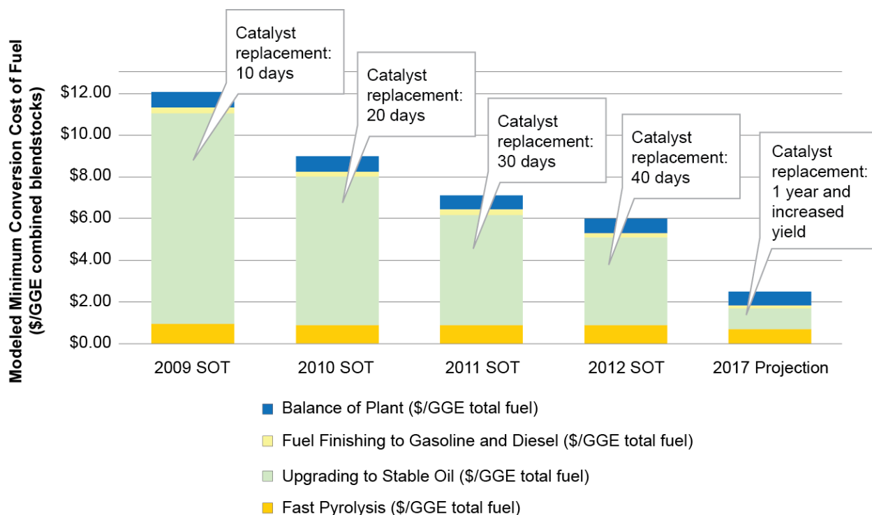
Figure 2-23: Conversion of woody feedstocks to renewable gasoline and diesel finished fuels via fast pyrolysis
