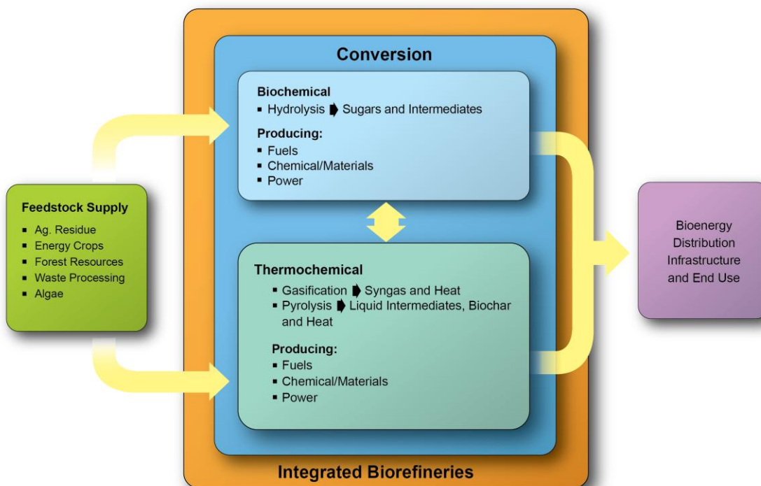
Figure 2-16: Conversion routes for biomass to bioenergy
