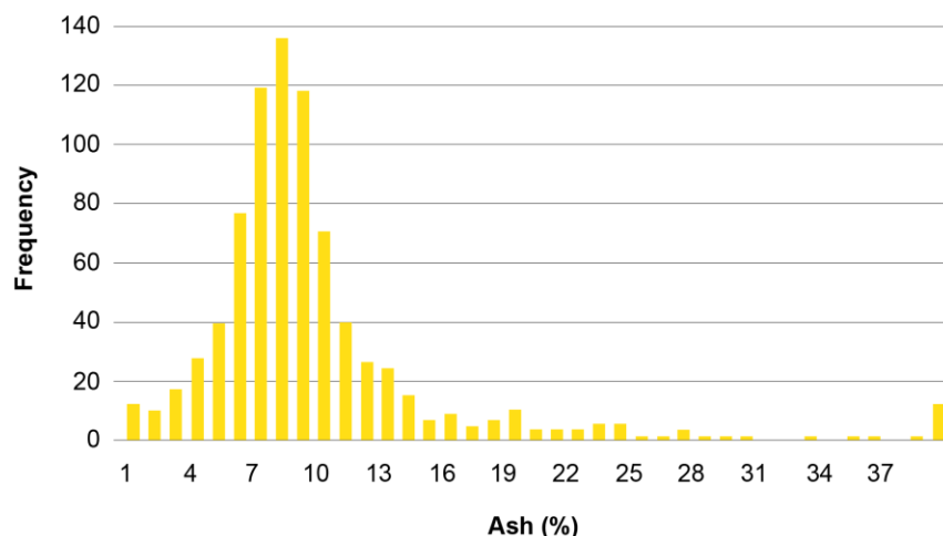
Figure 2-8: Demonstration of the variability in total ash content in corn stover 20
