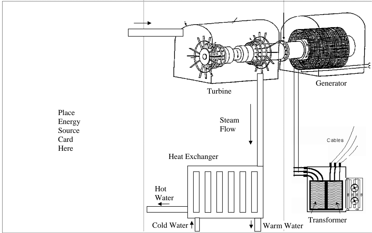
Overhead of Power Plant 5x8 Schematic
