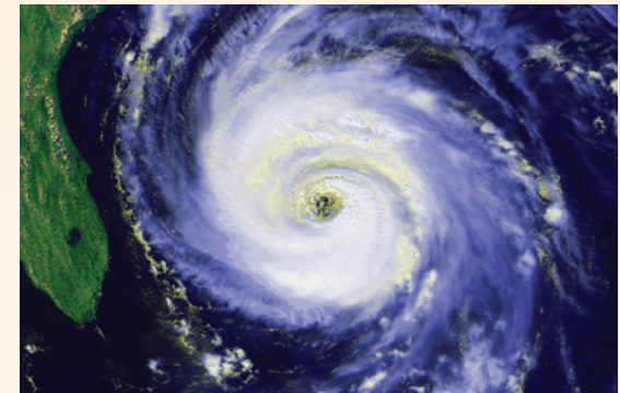
Storms like this hurricane are powered by the latent heat energy of water as it changes phase from liquid to gas, and then back to liquid. (Source: National Oceanic and Atmospheric Administration, Environmental Visualization Laboratory)
