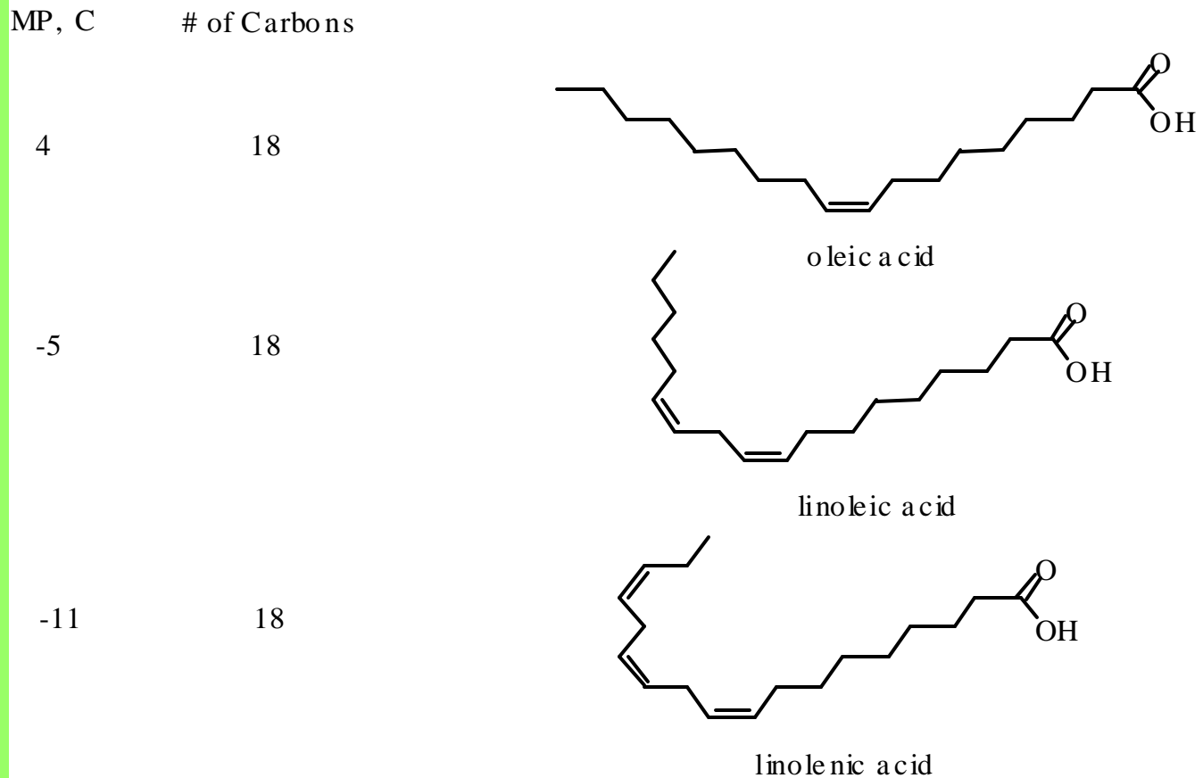
Structures and Properties of Some Unsaturated Fatty Acids
