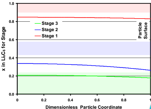
Li Concentration Distribution in Graphite Particle 1000s into C/1 Discharge
