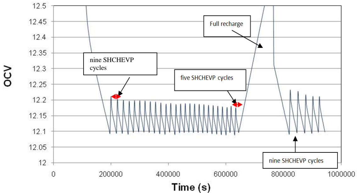
Figure 15. Typical open-circuit voltage of a Furukawa UltraBattery (ETA-134) operating under the Simulated Honda Civic Hybrid Electric Vehicle Profile, with a state-of-charge window of 43 to 53%.
