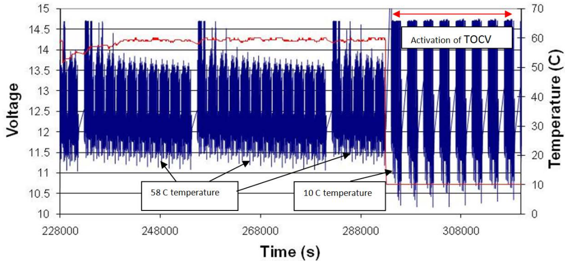
Figure 21. Typical voltage of a Furakawa UltraBattery (ETA-134) operating under the Simulated Honda Civic Hybrid Electric Vehicle Profile at battery temperatures of 58°C (136°F) and 10°C (50°) (state-of-charge window of 43 to 53%).
