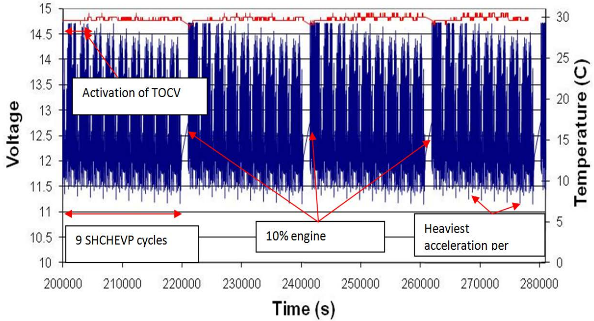
Figure 14. Typical voltage of a Furukawa UltraBattery (ETA-134) operating under the Simulated Honda Civic Hybrid Electric Vehicle Profile, with a state-of-charge window of 43 to 53% and battery temperature of 30°C (86°F).
