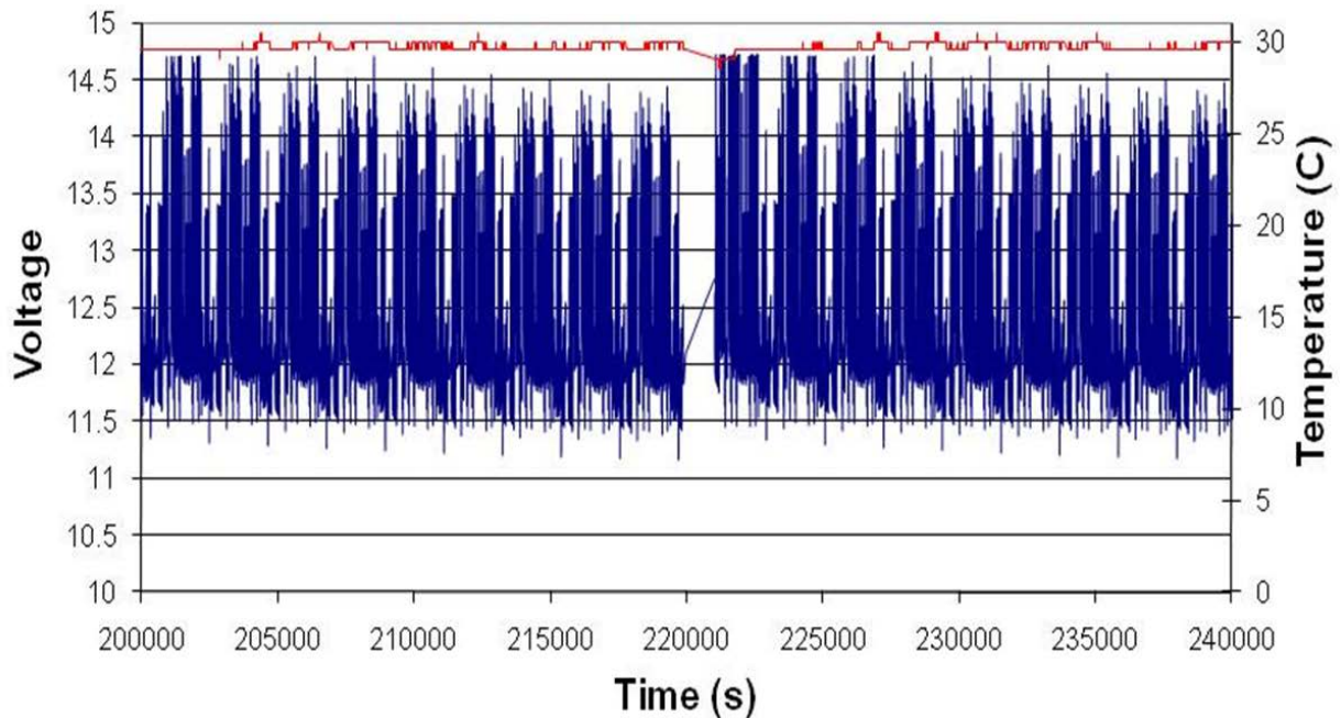
Figure 20. Typical voltage of a Furakawa UltraBattery (ETA-134) operating under the Simulated Honda Civic Hybrid Electric Vehicle Profile at a battery temperature of 30°C (86°F) (state-of-charge window of 43 to 53%).
