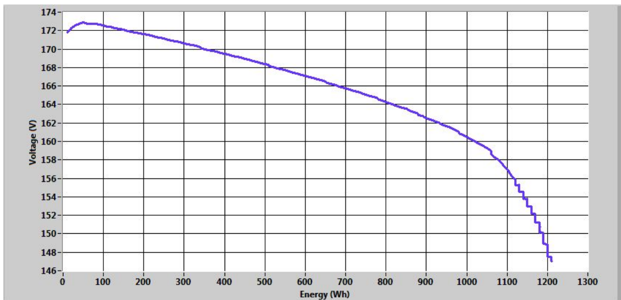
Figure 1: Voltage vs. Energy Discharged
