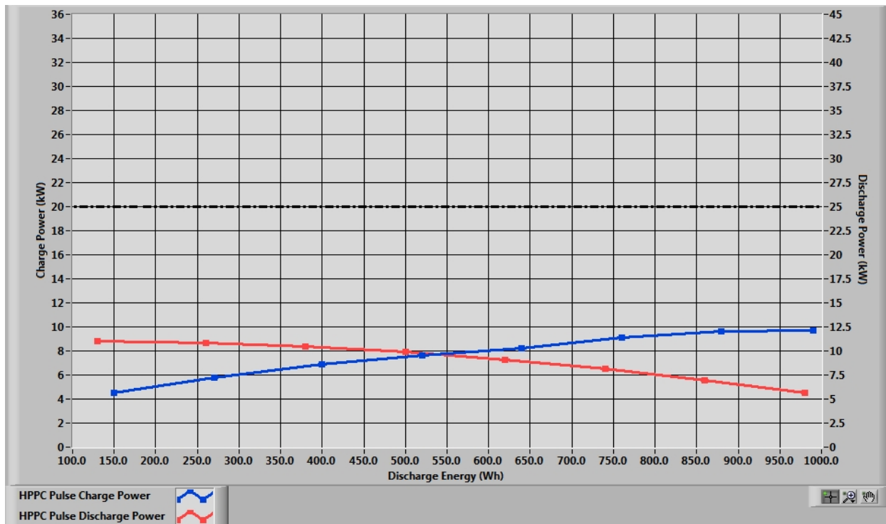
Figure 6: Peak Power Values with DOE Performance Goals
