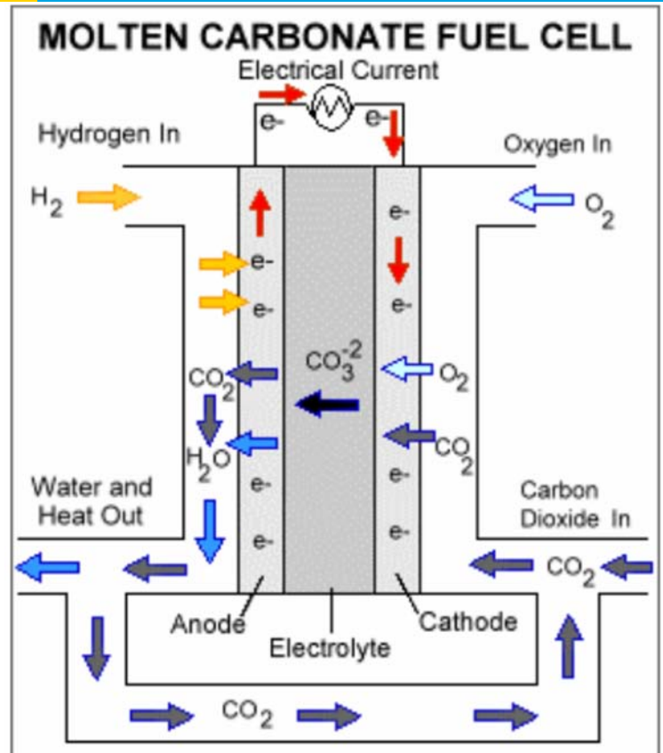
Schematic of a molten carbonate fuel cell
