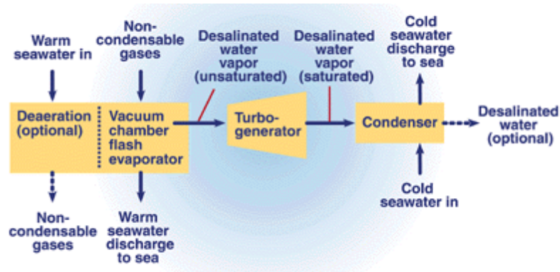
Figure A-7. Open loop cycle OTEC
