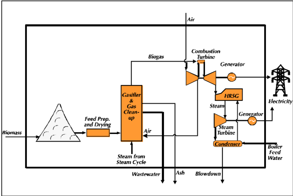
Figure A-2. Example of gasification combined cycle system
