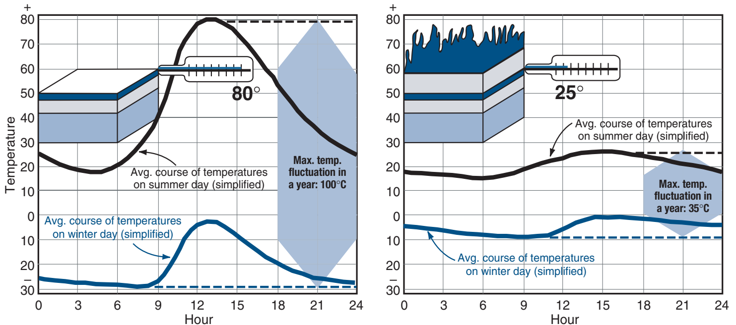
In the graph on the left, the arrow shows the maximum temperature fluctuation of a typical flat conventional roof, up to 60°C (140°F) in a single day, and up to 100°C (212°F) during the year. The graph on the right shows a significantly lower temperature fluctuation on a green roof. The protective green-roof layer moderates temperature extremes and protects the roofing membrane from accelerated aging caused by UV radiation. 7 (Source: A. Dürr, 1995; adapted with permission)
