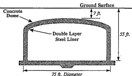
Figure S.2.2 Tank Schematic
