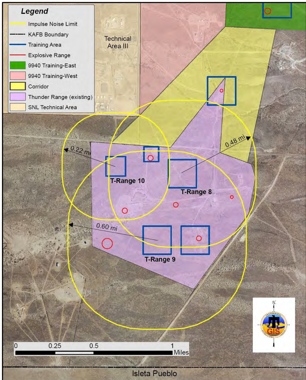
FIGURE 4.4-4 Impulse Noise Limits for Maximum Unmitigated Explosive Quantities at T-Ranges 8, 9, and 10, and Relationship to Nearby Receptors
