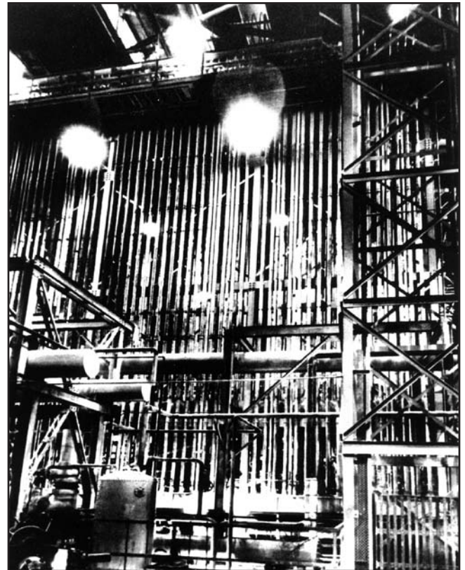
Section of S-50 Liquid Thermal Diffusion Plant at Clinton. Reprinted from Richard G. Hewlett and Oscar E. Anderson, Jr., The New World, 1939-1946 , Volume I of A History of the United States Atomic Energy Commission (University Park: Pennsylvania State University Press, 1962).
