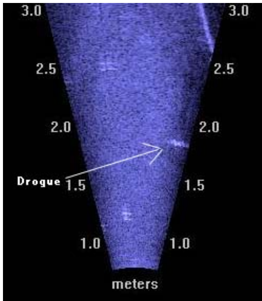
Figure 28. DIDSON image, recorded at 2.0 MHz, of a drogue released into the flume at an induced flow rate of 3.0 mps.
