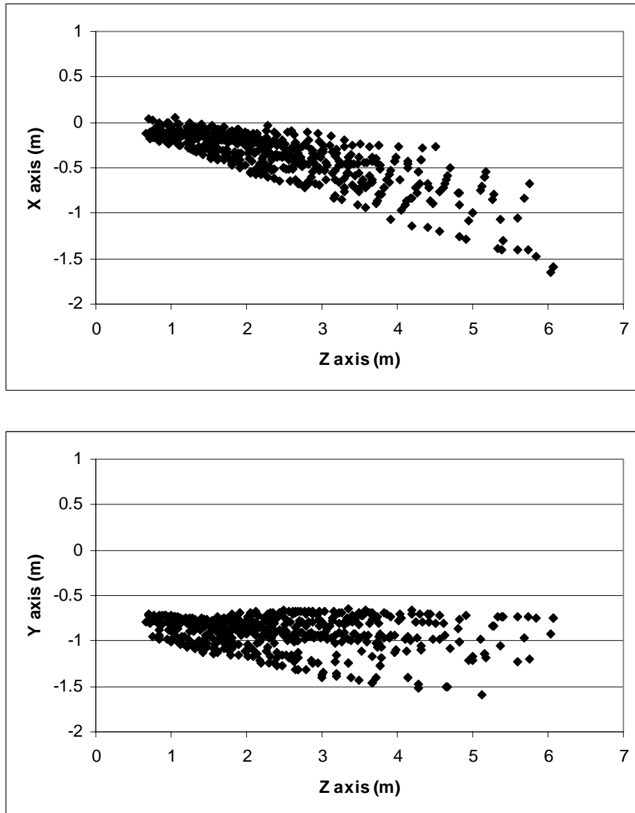
Figure 12. Trajectory of all LED drogues released into a turbine intake at McNary Dam at 60 MW load in the (a) X-Z plane and (b) Y-Z plane tracked with all six pairs of camera combinations. (Study conducted by PNNL for Walla Walla District USACE.)
