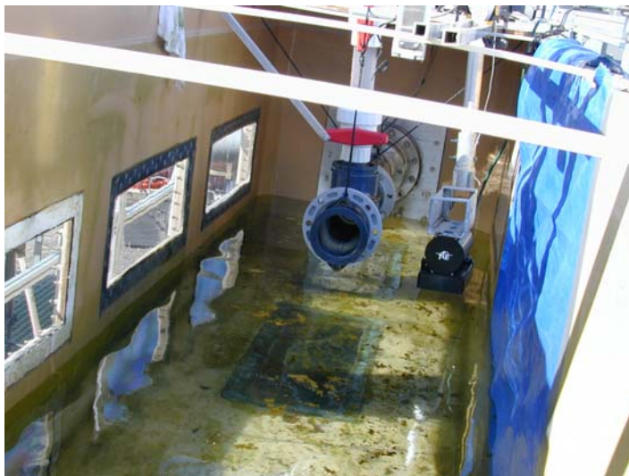
Figure 5. Induction pipe (left) and DIDSON (right) mounted in the test flume.
