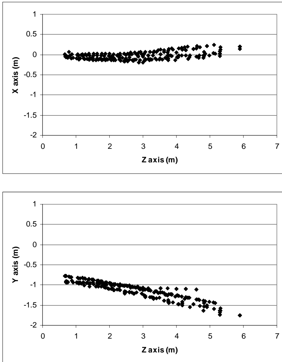
Figure 10. Trajectory of an individual LED drogue as it passed through a turbine intake at McNary Dam in the (a) X-Z plane and (b) Y-Z plane tracked with all six pairs of camera combinations. The different paths of the LED drogue are due to error in orientation of the pairs of cameras used to calculate drogue trajectory. With four cameras used six trajectories were calculated using all combinations of camera pairs. (Study conducted by PNNL for Walla Walla District USACE.)
