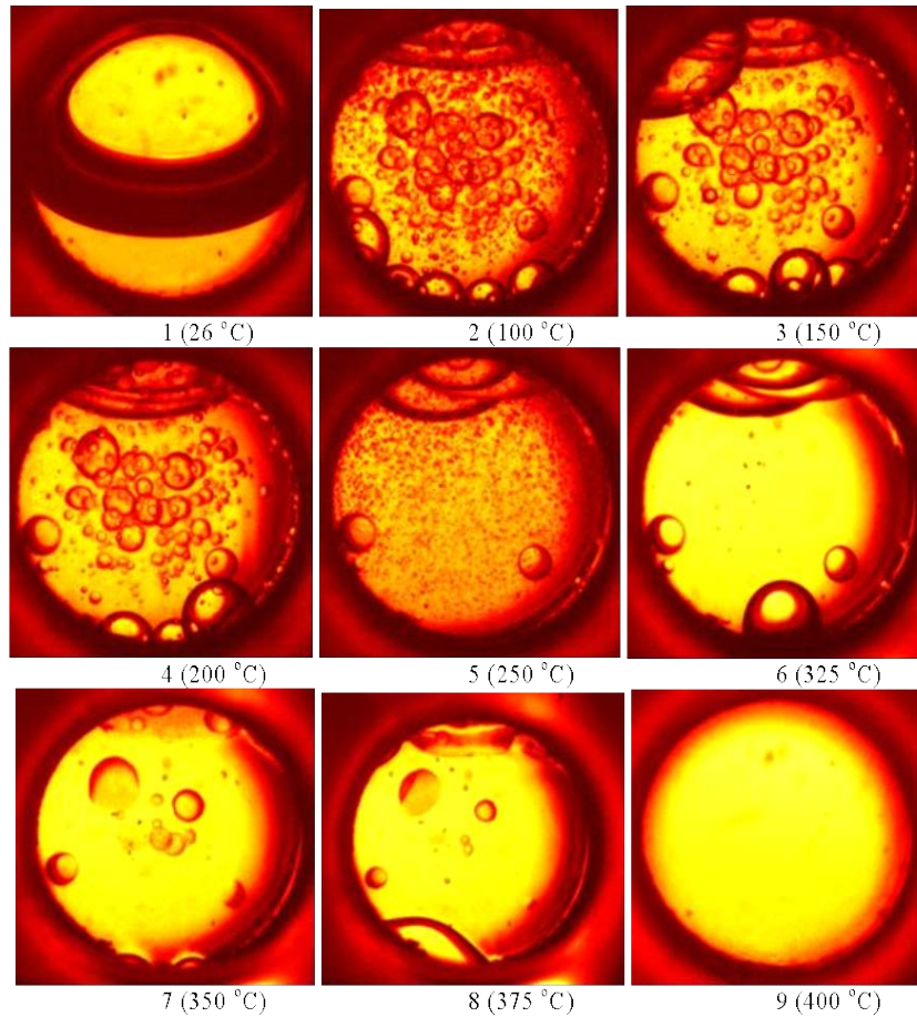
Miscibility of soybean oil and ethanol
